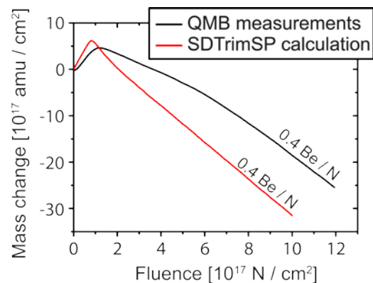
Fig. 2 Mass change of the Be-covered quartz crystal as a function of N fluence: Comparison of the QMB measurements to dynamic calculations with SDTrim.SP. The inserts show an exploded view of the QMB setup and a photograph of four Be-coated quartz crystals with gold rims.
