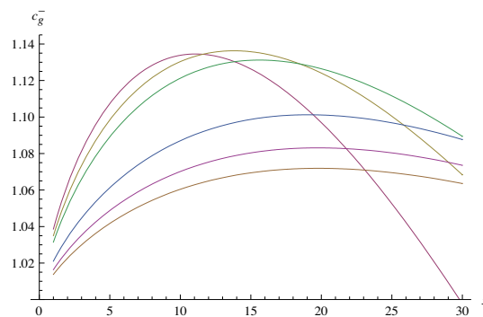
Figure 4. c_g^- is plotted against x \equiv \left(\frac{\lambda}{L} - \frac{1}{2}\right) \times 10^2 for (u, v) lying on the plane (2.18). Different colors correspond to different values of v = 2, 3, 5, 10, 15, 20 . The group velocity is found to exceed unity.
