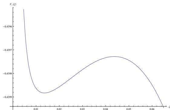
Figure 1. V_-(\zeta) is plotted for \tilde{k} = 10^8, v = 1, w = 1 and \lambda = 0.6 , subject to the conditions (2.18)–(2.19). The potential develops a well close to the boundary. V_+(\zeta) has an identical plot with the sign of \lambda flipped.
