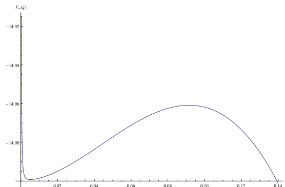
Figure 2. V_-(\zeta) is plotted for \tilde{k} = 10^8, v = 1, w = 1 and \lambda = 2.0 , subject to the conditions (2.18)–(2.19). The potential develops a well close to the boundary. V_+(\zeta) has an identical plot with the sign of \lambda flipped.
