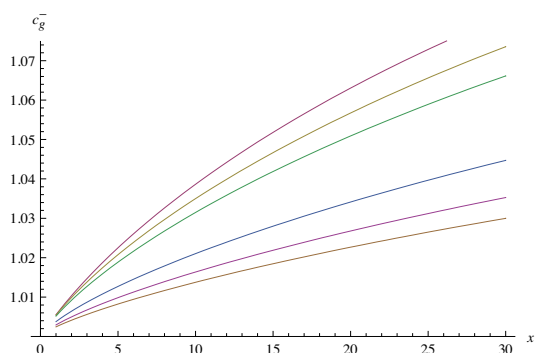
Figure 3. c_g^- is plotted against x \equiv \left(\frac{\lambda}{L} - \frac{1}{2}\right) \times 10^3 for (u, v) lying on the plane (2.18). Different colors correspond to different values of v = 2, 3, 5, 10, 15, 20 . The group velocity is found to exceed unity.
