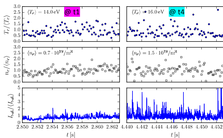
Figure 4: Langmuir probe data, T_e (top), n_e (middle) and I_{\text{sat}} (bottom), from two different time periods: left, time point t_1 but without type-I ELMs, right: t_4 is a mitigated phase at high fuelling level. All values are normalized to their mean.
