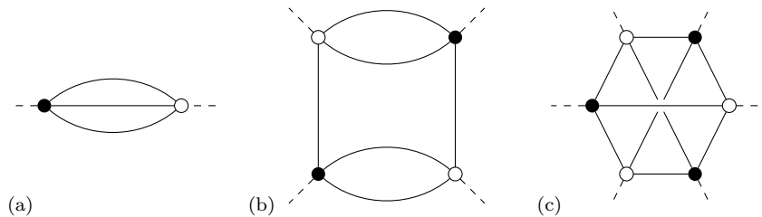
FIG. 1. Three examples of Feynman graphs for a rank 3 TGFT's. The trace invariants used to build the interactions are: figure (a) \text{Tr}(\bar{\phi}\phi) , figure (b) an example of \text{Tr}(\bar{\phi}\phi\bar{\phi}\phi) , figure (c) an example of \text{Tr}(\bar{\phi}\phi\bar{\phi}\phi\bar{\phi}\phi) .
