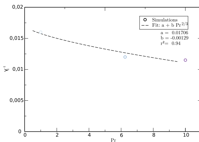
Figure 5. Simulated \gamma as extrapolated from Figure 4 for Le \approx 200 (circles) and power law prediction by McPhee et al. [1987] (dashed line). Colors indicate different Prandtl numbers: Pr = 1 (light blue), Pr = 6.25 (blue), and Pr = 10 (purple).
