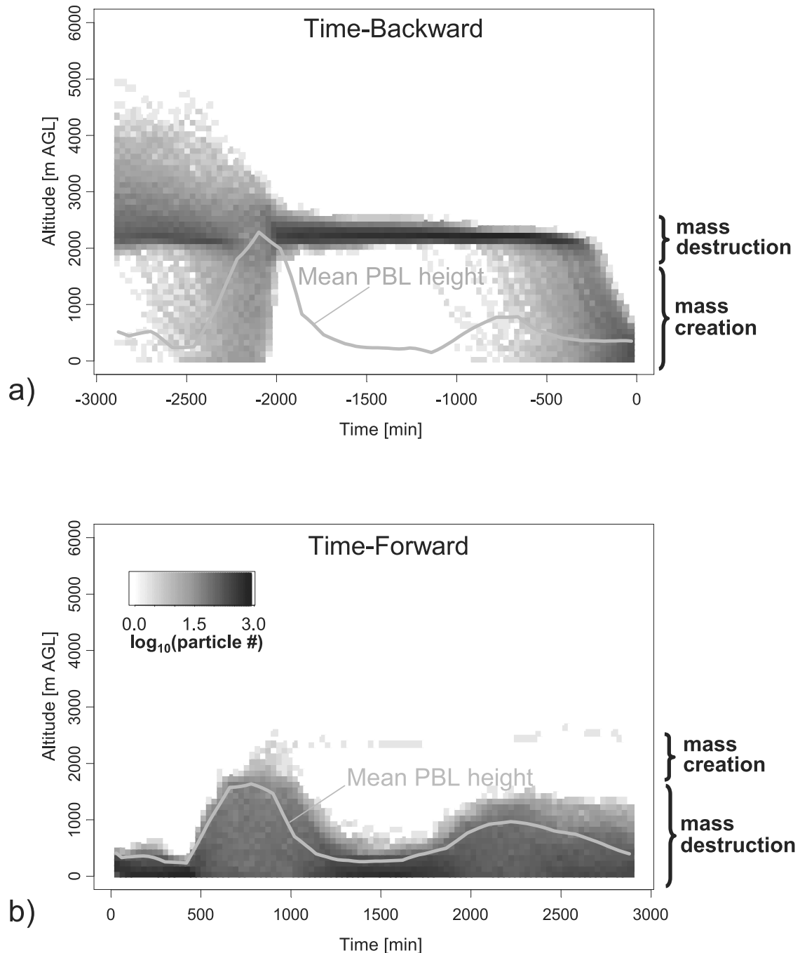
Figure 5. Particle runs driven with mass-violating wind fields in a simplified atmosphere. Particle simulations (a) backward and (b) forward in time, driven by winds with 15% mass violation below 1800 m above ground level and >100% between 1800 and 2200 m.
