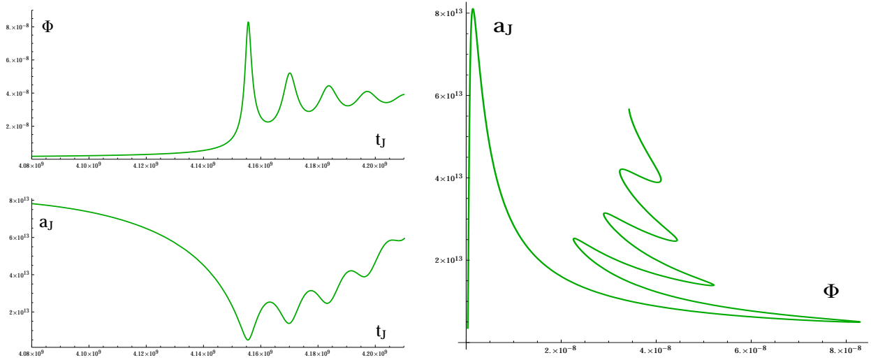
FIG. 5: Left: Scalar field and scale factor for the transformed solution in Jordan frame. Right: Parametric plot of the scalar field and scale factor in Jordan frame. As the scalar field stabilises, the scale factor goes through oscillations as well, but eventually increases monotonically.
