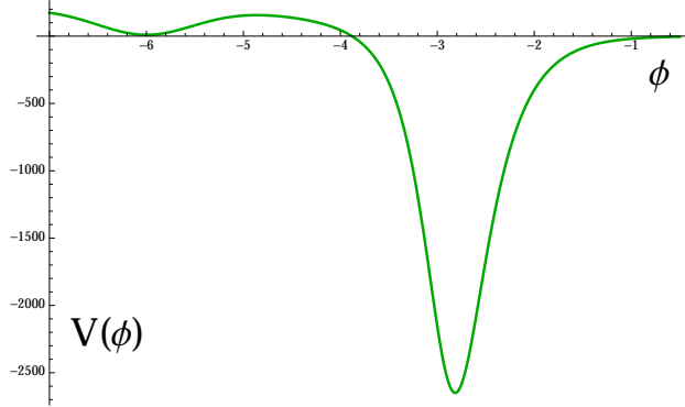
FIG. 3: The Einstein frame scalar potential used in the bounce model (33).
