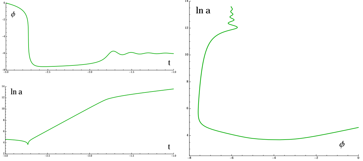
Figure 4. Left: scalar field and scale factor for the bounce solution in Einstein frame. Right: parametric plot of the scalar field and scale factor in Einstein frame. This plot nicely illustrates the smoothness of the bounce.
