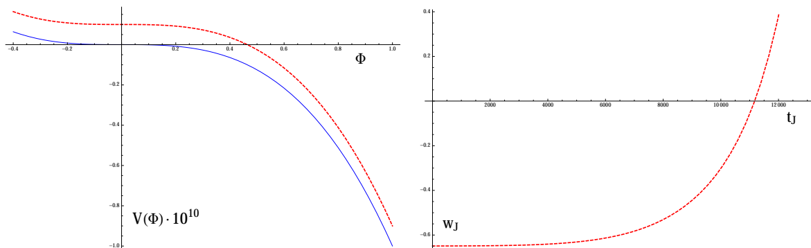
Figure 1. Left: the original Jordan frame potential V_J is shown in blue, the shifted potential U_J in dashed red. Right: the equation of state in Jordan frame, for the shifted potential.
