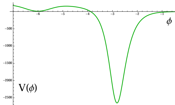
Figure 3. The Einstein frame scalar potential used in the bounce model (3.30).
