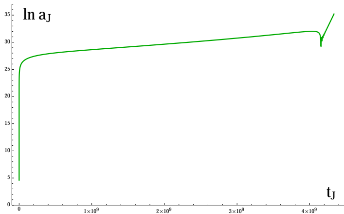
Figure 5. Full evolution of the scale factor for the transformed solution in Jordan frame. The conflationary phase lasts while the scalar field rolls up the potential towards \Phi \sim 10^{-9} . During this period the scale factor increases by many orders of magnitude. During the exit of the conflationary phase the scale factor and scalar field undergo non-trivial evolution which is hard to see in the present figure and is shown in detail in figure 6.
