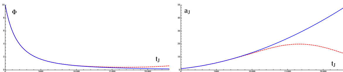
Figure 2. Scalar field and scale factor in Jordan frame: the blue curves show the transformed ekpyrotic scaling solution and the red dashed curves correspond to the field evolutions in the shifted potential.
