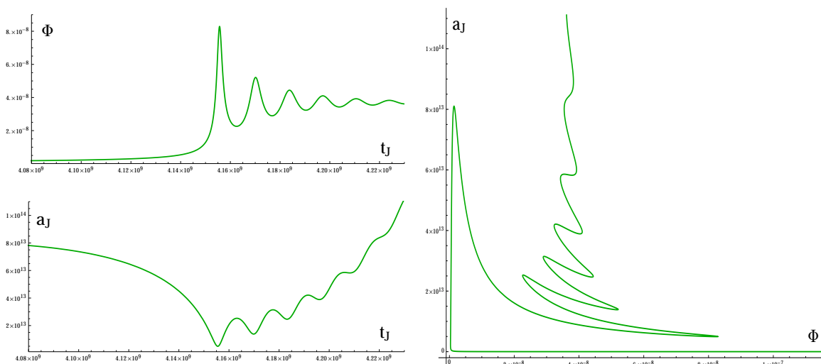
Figure 6. Left: scalar field and scale factor for the transformed solution in Jordan frame towards the end of the evolution. Right: parametric plot of the scalar field and scale factor in Jordan frame. Note that initially the scalar field decreases its value very rapidly. Later on as the scalar field stabilises, the scale factor goes through oscillations, but eventually increases monotonically.
