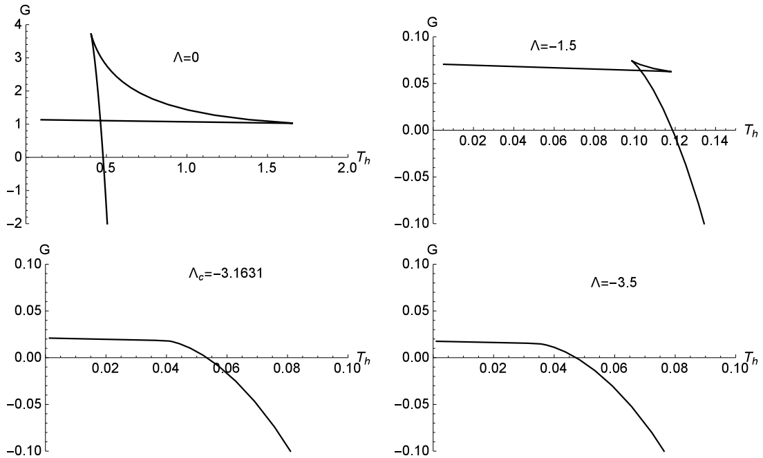
Figure 7: When \alpha = 1 , \eta = 2 , and q = 0.3 , plots of the relation of G with respect to T_h for different values of \Lambda .
