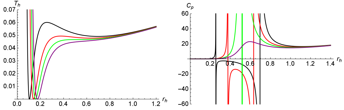
Figure 4: When \alpha = 1 , \eta = 2 , and \Lambda = -1.5 , plots of the relations of T_h and C_p with respect to r_h for q = 0.3 (Black), q = 0.4 (Red), q_c = 0.45049 (Green), and q = 0.5 (Purple), respectively.
