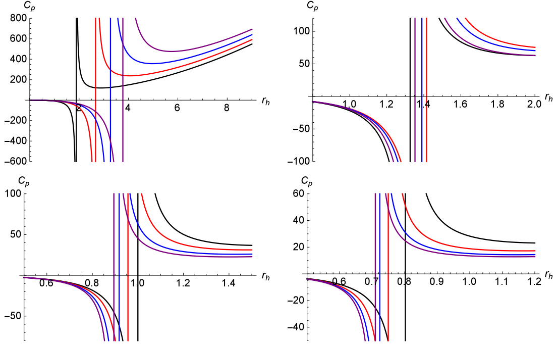
Figure 2: When \alpha = 1 , plots of the relation of C_p with respect to r_h for \eta = 1 (Black), 2 (Red), 3 (Blue), and 4 (Purple) at \Lambda = 0 (top left), \Lambda = -0.5 (top right), \Lambda = -1 (bottom left), and \Lambda = -1.5 (bottom right), respectively.
