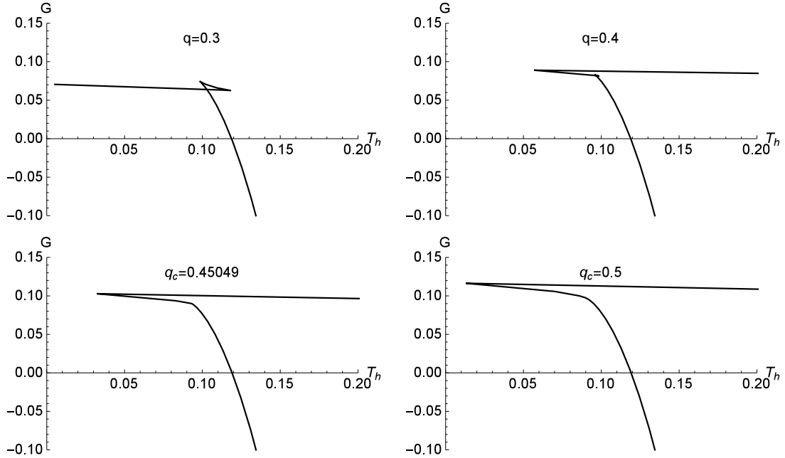
Figure 6: When \alpha = 1 , \eta = 2 , and \Lambda = -1.5 , plots of the relation of G with respect to T_h for different values of q .
