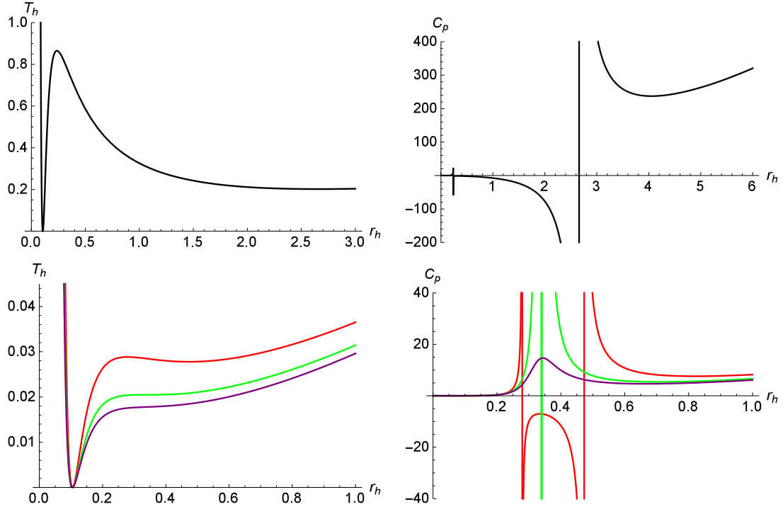
Figure 5: When \alpha = 1 , \eta = 2 , and q = 0.3 , plots of the relations of T_h and C_p with respect to r_h for \Lambda = 0 (Black), \Lambda = -2.5 (Red), \Lambda_c = -3.1631 (Green), and \Lambda = -3.5 (Purple), respectively.
