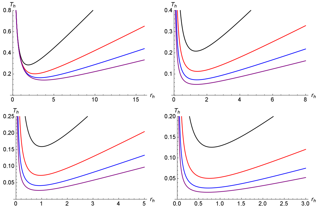
Figure 1: When \alpha = 1 , plots of the relation of T_h with respect to r_h for \eta = 1 (Black), 2 (Red), 3 (Blue), and 4 (Purple) at \Lambda = 0 (top left), \Lambda = -0.5 (top right), \Lambda = -1 (bottom left), and \Lambda = -1.5 (bottom right), respectively.
