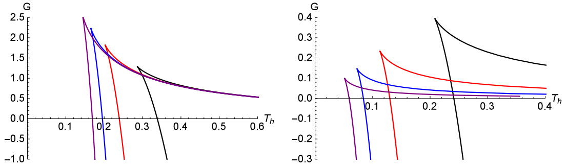
Figure 3: When \alpha = 1 , plots of the relation of G with respect to T_h for \eta = 1 (Black), 2 (Red), 3 (Blue), and 4 (Purple) at \Lambda = 0 (left) and \Lambda = -0.5 (right), respectively.
