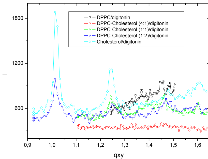
Fig. S2. GIXD patterns for DPPC, cholesterol and their mixed monolayers compressed to \Pi_0 = 32.5 mN/m on digitonin ( 10^{-4} M)
