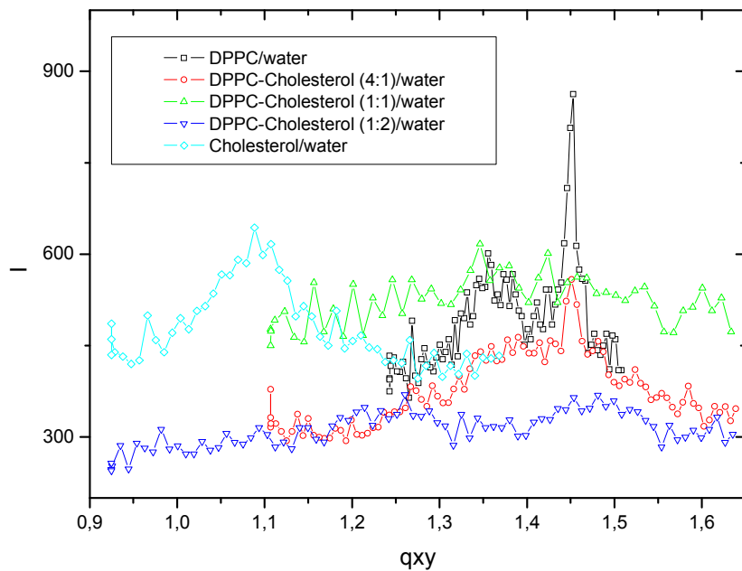
Fig. S1. GIXD patterns for DPPC, cholesterol and their mixed monolayers compressed to \Pi_0 = 32.5 mN/m on water.
