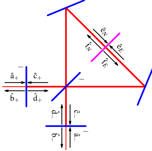
FIG. 3. To calculation of optical fields in the Michelson-Sagnac interferometer.
