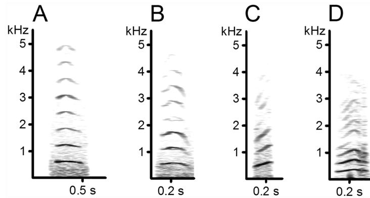
Fig 1. Spectrograms of rhesus female coo calls. Coo call of subject A and B have a relatively high similarity (i.e., a low F-value of 0.97), whereas the coo calls of subject C and D have a low similarity (high F-values of 6.71). F-values for the other combinations: A vs. C = 4.5, A vs. D = 3.7, B vs. C = 4.63, B vs. D = 3.81.
