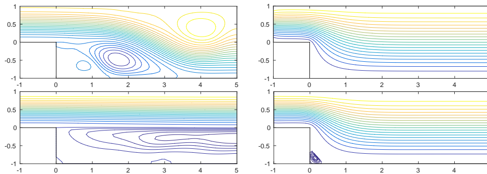
FIG. 11. Vorticity plots at t = 12 (top) and t = 200 (bottom) for the forward (uncontrolled) Navier–Stokes system (left), and the controlled system with the minimized vorticity (right).
