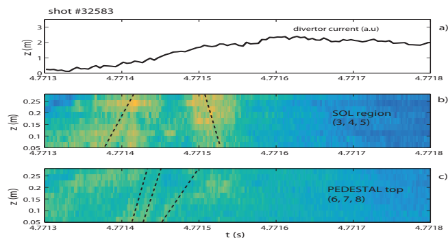
Figure 5: a) Divertor current. Averaged temperature fluctuations for different radial channels shown in: b) the SOL region; c) the pedestal top
