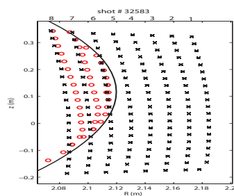
Figure 4: Cold and warm resonance positions for the shot #32583 just before an ELM crash
