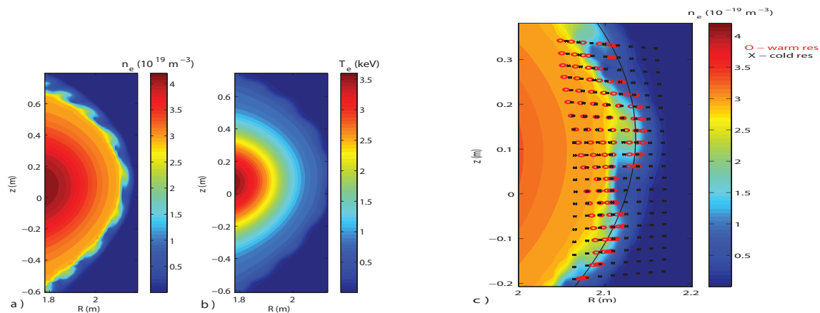
Figure 3: 2D JOEREK profiles of a) Electron density; b) electron temperature. These profiles are adjusted to the actual values of the density and the temperature for the shot # 33195 at time t = 2.5872 s and used as an input for ECFM. c) Warm resonance positions as calculated with the ECFM (O); Cold resonance positions along the LOS (X).
