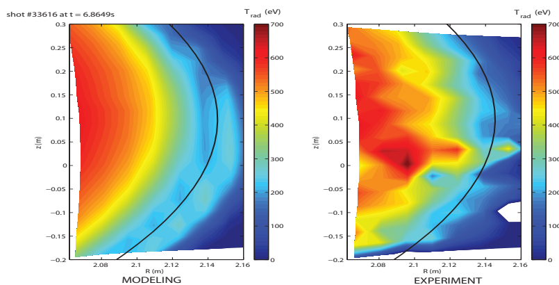
Figure 2: Radiation temperature ( T_{rad} ) a) Modelled radiation temperature without the presence of the instabilities. b) Measured radiation in the ELM free interval. Measurement positions correspond to the cold resonances. Black lines represent the separatrix position.
