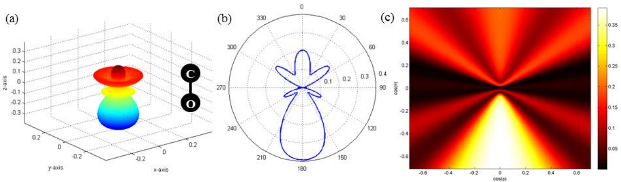
Figure 2. Photoelectron diffraction pattern for C(1s) photoelectron emission from CO molecules at 300 eV photoelectron kinetic energy and for ionization with linearly polarized X-rays with the polarization vector along the molecular axis, which is along the z-axis. (a) Full three-dimensional photoelectron angular distributions. (b) Polar plot of the photoelectron intensity in the xz-plane as a function of the emission angle \theta (c) Two-dimensional (2D) projection of the photoelectron angular distribution onto the xz-plane as it would be recorded by a 2D imaging detector placed parallel to the molecular axis in the far field. For this model calculation, the amplitudes A and B in eq. (4) are assumed to be A=B=1.
