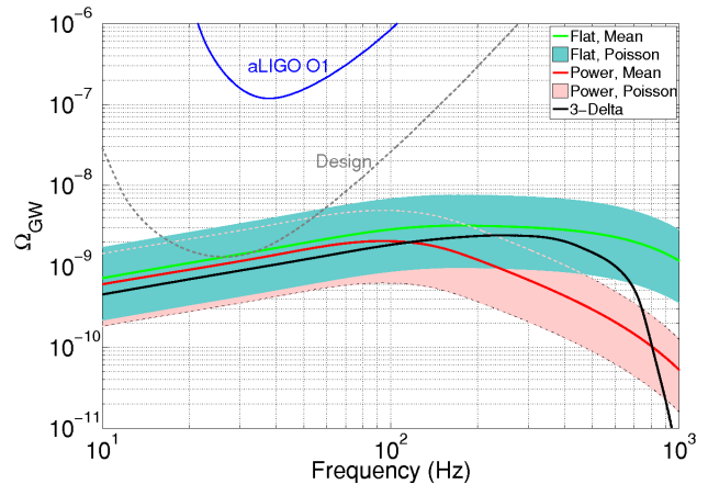
FIG. 5. We present a range of potential spectra for a BBH background, using the flat-log, power-law, and 3-delta mass distribution models described in [44, 67], with the local rate inferred from the O1 detections [44]. For the flat-log and power-law distributions, we show the 90% Poisson uncertainty band due to the uncertainty in the local rate measurement. In addition, we show the measured O1 PI curve and the projected PI curve for Advanced LIGO-Virgo operating at design sensitivity.
