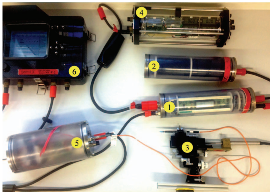
Fig. 1. Diver-operated microsensors system (DOMS) with (1) the measurement control and data storage module, (2) the battery, (3) the motorized micromanipulator equipped with the spectral scalar irradiance microsensors (orange fiber), (4) the commercial underwater PAR meter, (5) the underwater module containing the Ocean Optics spectrometer, and (6) the underwater personal computer module. Modules (1–3) were part of the original design developed by Weber et al. (2007); modules (5 and 6) were designed and developed during this study.
