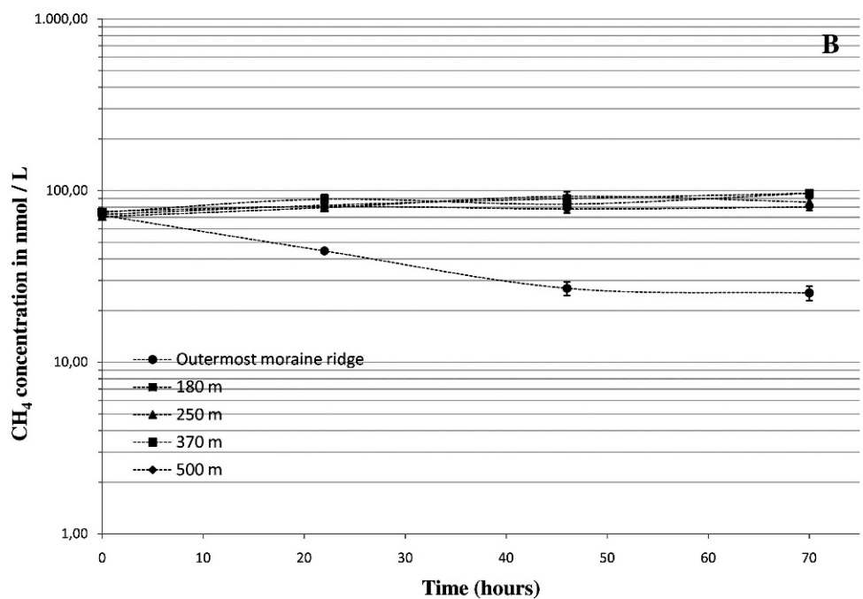
FIGURE 3. (A) Semilogarithmic plot of CH 4 headspace concentrations over 98 hours. Incubation temperature 22 °C. Plotted values are means, error bars indicate \pm SE ( n = 4 ). (B) Semilogarithmic plot of CH 4 headspace concentrations over 70 hours. Incubation temperature 10 °C. Plotted values are means, error bars indicate \pm SE ( n = 4 ).
