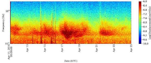
FIG. 13. Spectrogram of seismic noise in the 0.1 Hz~2 Hz band during the second run. One can see large spikes on April 14th and 16th due to a series of large earthquakes in Kumamoto. Some data on April 17th and 21st is missing due to an issue in our data taking system.
