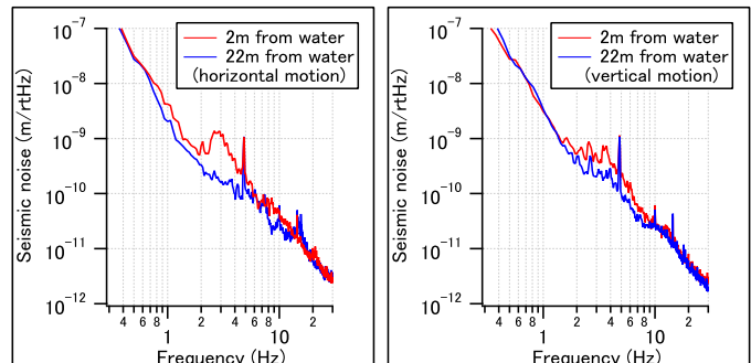
FIG. 15. Seismic noise measured at two locations near the Y-end chamber; one is close to the drain pipe and the other far away from the drain pipe.
