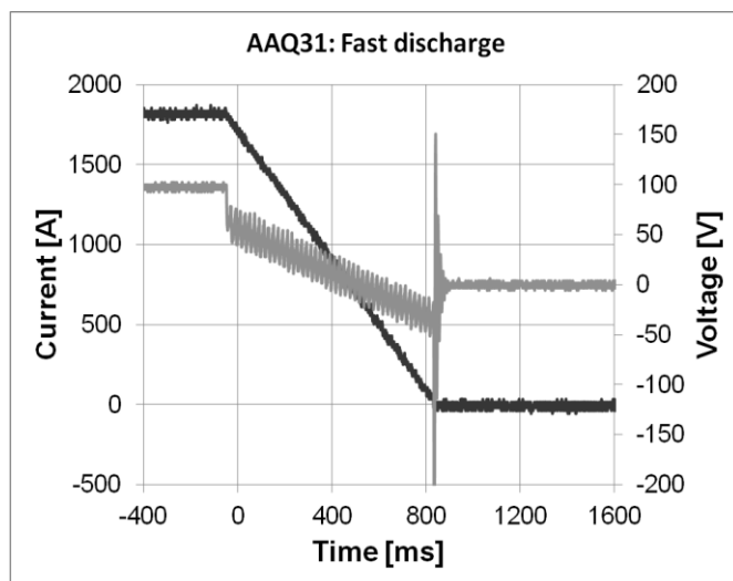
Fig. 5. Fast discharge of a trim coil after the modification of the discharge control system (current: black; voltage: grey).
