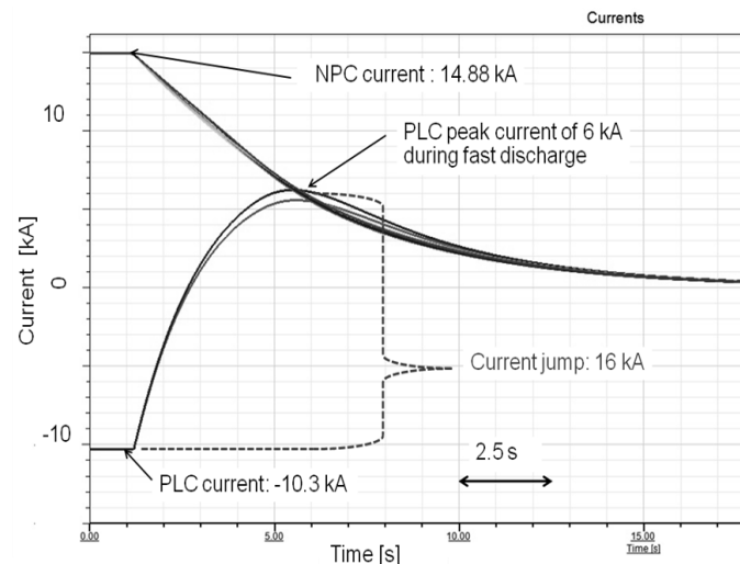
Fig. 4. Currents in the non-planar and the planar coils before and during a fast discharge (modified dump resistor).
