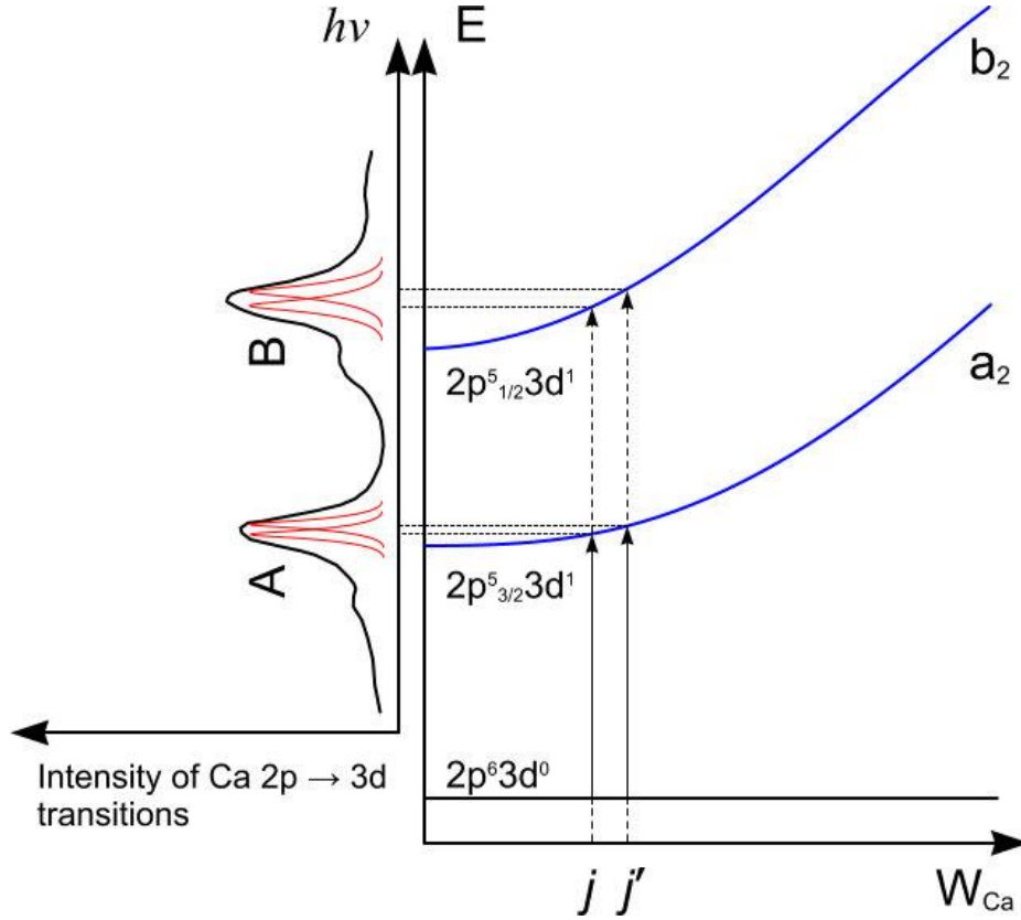
Figure 3. Schematic presentation of the surroundings effect on the A and B line shape in mineralized bone.
