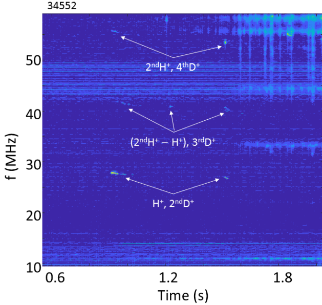
FIG. 4. ICE frequency spectrum for the discharge shown in Fig. 3 (a)-(d).
