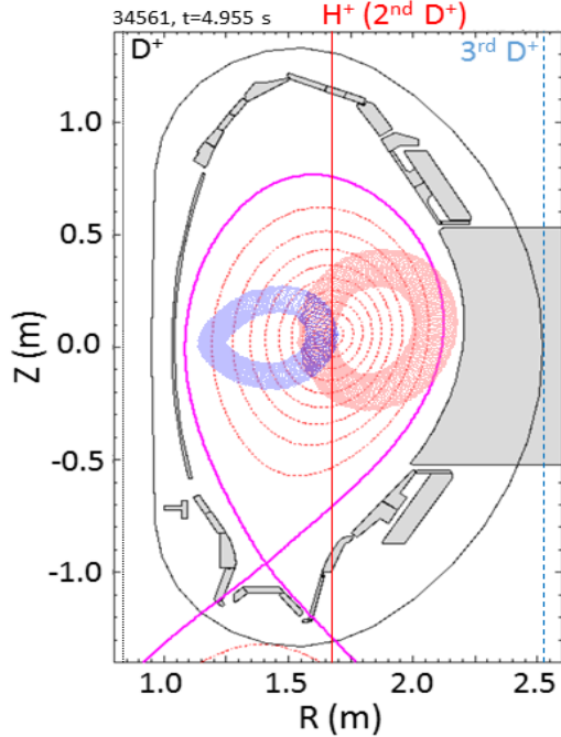
FIG. 6. Frequency matched radial positions of the fundamental deuterium (dotted black line), the fundamental hydrogen (solid red line), and the third harmonic deuterium (dashed blue line) cyclotron frequencies for discharge shown in FIG. 5. The two shown orbits correspond to barely confined fusion proton orbits. Both orbits originate at the magnetic axis.
