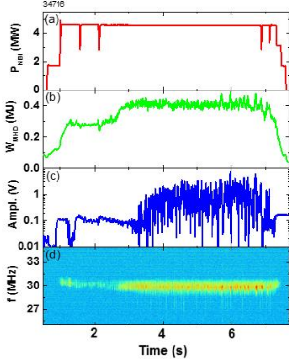
FIG. 2. A “classic” ICE example of low field side edge emission due to NBI fast ions on ASDEX Upgrade (discharge #34716, B_T = -2.47 T, H plasma, H beams). The plotted quantities are (a) the NBI power P_{\text{NBI}} ; (b) the stored plasma energy W_{\text{MHD}} ; (c) the RF probe amplitude on the low field side, on a logarithmic scale; and (d) the measured ICE intensity frequency spectrum f , on a logarithmic scale (see (c) for relative scale).
