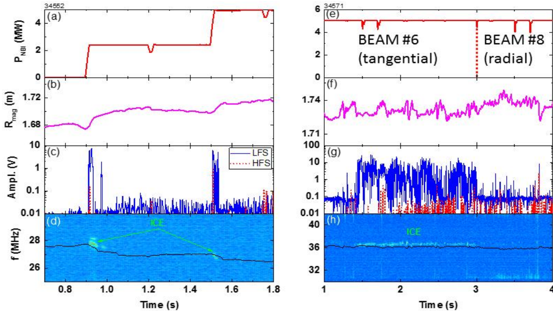
FIG. 3. Examples of core ICE at B_T = -1.79 T (discharge #34552, (a)-(d)) and B_T = -2.47 T (discharge #34571, (e)-(h)). D plasma and D beams. The plotted quantities are the NBI power P_{\text{NBI}} (a) and (e); the radial position of the magnetic axis R_{\text{mag}} (b) and (f); the amplitude of the RF signal on the low and the high field sides (LFS and HFS), on a logarithmic scale (c) and (g); and the frequency spectra of measured ICE intensity, on a logarithmic scale (d) and (h) (see (c) and (g) for relative scales, respectively). The black lines in (d) and (h) indicate the fundamental hydrogen cyclotron frequency calculated at the magnetic axis.
