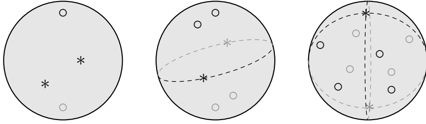
Figure 2: The compactified complex plane for z , x or y , respectively. The points corresponding to z_{\pm}^{\circ} = 0, \infty are marked by \circ . The self-dual points corresponding to z_{\pm}^* are marked by * . The spheres are divided into one, two or four regions which are identified by a twist.
