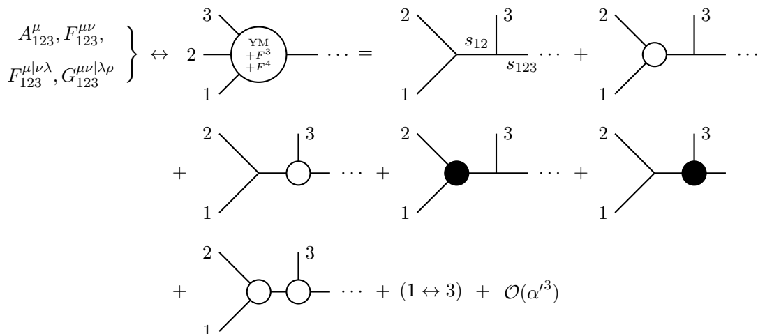
Figure 7. Berends-Giele currents A_{12\dots p}^\mu , F_{12\dots p}^{\mu\nu} , F_{12\dots p}^{\mu|\nu\lambda} and G_{12\dots p}^{\mu\nu|\lambda\rho} of rank p combine the diagrams and propagators expected in a color-ordered (p+1) -point tree amplitude of (\text{YM}+F^3+F^4) with an off-shell leg. . . . Vertices marked with a white and black dot represent the first and second order in \alpha' on the right hand side of (3.11), i.e. the cubic-graph parametrization of \alpha'F^3 and \alpha'^2F^4 insertions.
