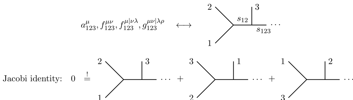
Figure 11. Diagrammatic interpretation of three-particle polarizations a_{123}^\mu, f_{123}^{\mu\nu}, f_{123}^{\mu|\nu\lambda}, and g_{123}^{\mu\nu|\lambda\rho} subject to kinematic Jacobi relations such as a_{123}^\mu + \text{cyc}(1, 2, 3) = 0 .
