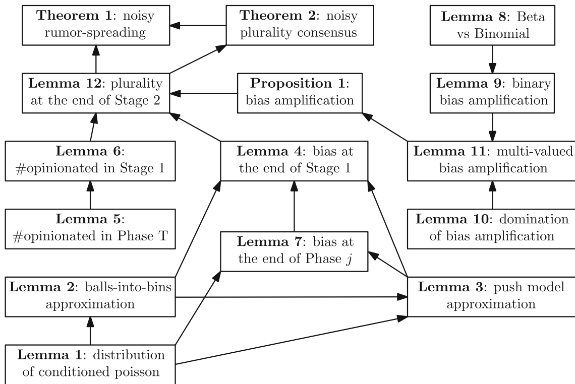
Fig. 1 Diagrams of dependencies among the different parts of the analysis. Each box represents a statement proven in the analysis, and an arrow between two boxes u and v signifies that the statement of box u is employed in the proof of box v
