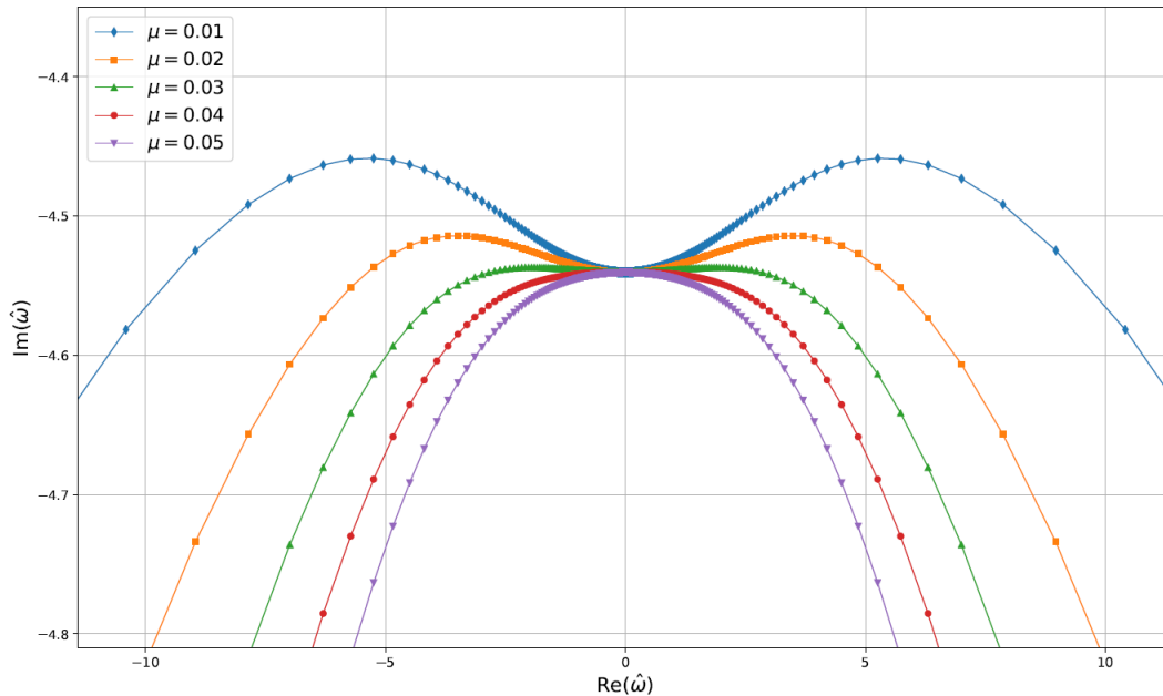
FIG. 1. Spectra for different values \mu , and p = 1 . For n = 1 , as \hat{J} goes over the real line, the curves start at the imaginary axis ( \hat{J} \rightarrow -\infty ), then acquire a positive real part, approach the north pole of the Riemann Sphere ( \hat{J} \rightarrow 0^- ), then pass through the pole and acquire a negative real part, and end again in the imaginary axis as \hat{J} \rightarrow +\infty . For n = -1 the locus is exactly the same but it is travelled “counter-clockwise”.
