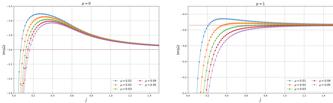
FIG. 3. Imaginary part of the frequency (always negative) as a function of the reduced angular momentum \hat{J} . For different values of \mu , and n = 1 . For large angular momentum the imaginary part of the frequencies approaches a finite constant. ( p = 0 left panel and p = 1 right panel).
