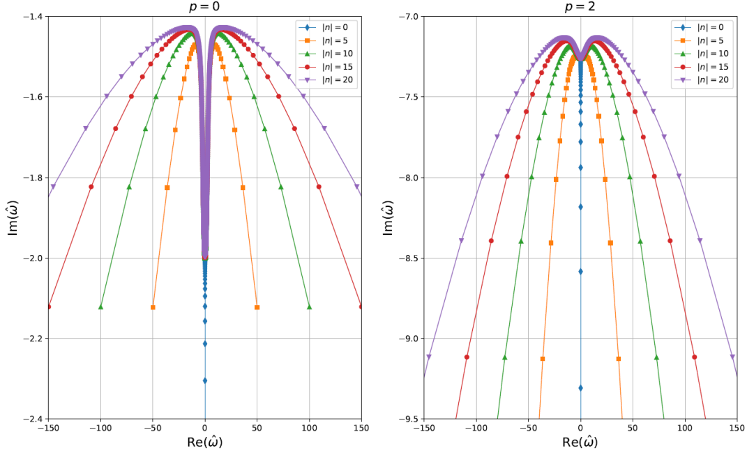
FIG. 2. Spectrum for different values of the azimuthal angular momentum of the scalar field. The circularly symmetric modes of the field ( n = 0 ) lie on the imaginary axis for any value of the angular momentum of the black holes which runs along the curves. We have fixed the gravitational hair as \mu = 0.01 and left panel shows the fundamental mode p = 0 while right panel shows the second existed modes with p = 2 . As expected, for a given value of the reduced angular momentum \hat{J} fixing the background, the modes with higher overtones have a higher damping.
