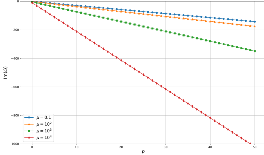
FIG. 5. Imaginary part of the frequencies as a function of the mode number p for different values of the gravitational hair parameter \mu . As the latter increases the modes acquire a higher damping. We have set \hat{J} = 10 and n = 1 .
