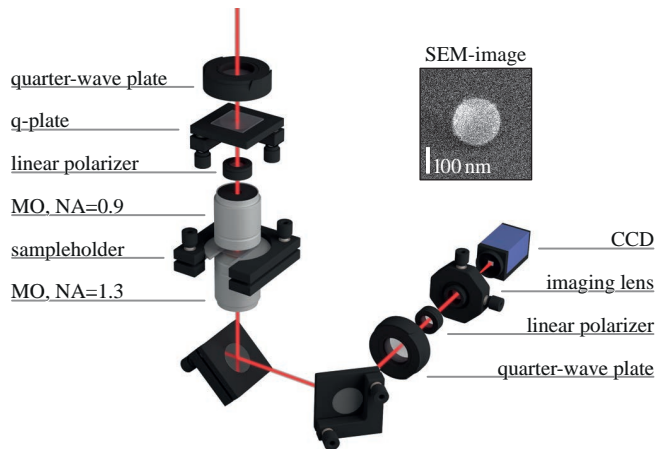
Figure 5. Sketch of the experimental setup. A quarter wave plate, a q-plate of charge -1/2 and a linear polarizer transform the incoming linearly polarized Gaussian beam into an LG_{\pm 1} mode. The paraxial beam is tightly focused onto a silicon nanoparticle (radius=87 nm, SEM-image shown as inset) by a microscope objective (MO). The light propagating in forward direction is collected by an immersion-type MO. A rotatable quarter-wave plate and a linear polarizer are utilized for polarization analysis before a lens images the back focal plane of the second MO onto a CCD-camera.
