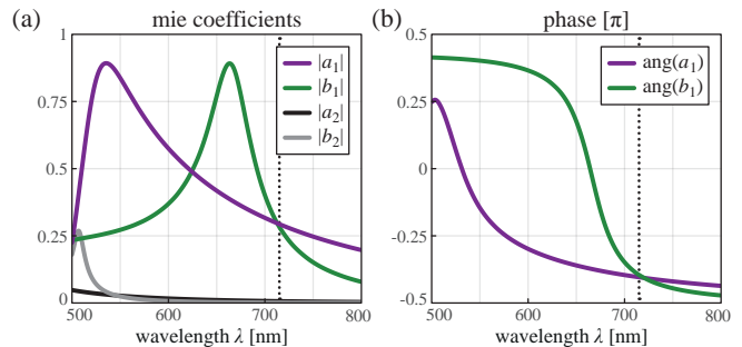
Figure 3. (a) Absolute values of the first and second order Mie coefficients of a core-shell nanoparticle with Si core of radius r_{\text{Si}} = 83 \text{ nm} and a \text{SiO}_2 shell of thickness \delta = 4 \text{ nm} . (b) Corresponding phases of the first order Mie coefficients. The dotted black lines show the wavelength \lambda_d = 715 \text{ nm} where the particle is approximately dual-symmetric, i.e. a_1 \approx b_1 .
