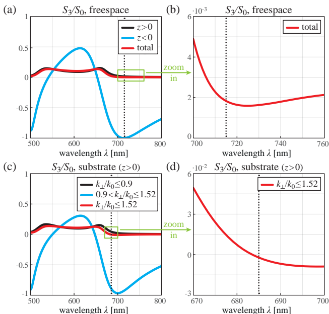
Figure 4. Scattering of a tightly focused LG_{+1} beam by the nanoparticle shown in Fig. 3. We show the average helicity ( S_3/S_0 ) of the emitted light by plotting the integrated Stokes S_3 parameter normalized by the integrated S_0 parameter. The wavelength \lambda_d where the particle is approximately dual-symmetric is indicated by dotted black lines. For free-space ( n_1 = n_2 = 1 ), (a) and (b) present the left half-space (blue), the right half-space (black) and the total value (red), where (b) shows an enlarged view onto the total value around \lambda_d . (c) and (d) show the case of the same scatterer positioned on a dielectric substrate ( n_1 = 1, n_2 = 1.52 ), where we integrate over the light emitted in forward direction over different angular regions. The blue, black and red curve show S_3/S_0 for 0.9 < NA_2 \leq 1.52 , NA_2 \leq 0.9 and NA_2 \leq 1.52 , respectively. (d) shows the area around \lambda_d in more detail.
