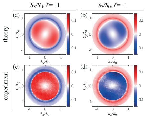
Figure 6. Theoretically calculated and experimentally measured back focal plane images of the second microscope objective. The colormap corresponds to the third Stokes parameter S_3 , normalized by the maximum of S_0 . (a) and (c) show the case of an azimuthal index \ell = +1 of the incoming LG mode, whereas (b) and (d) show results for \ell = -1 .
