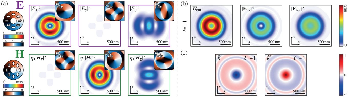
Figure 2. Calculated properties of an x -polarized LG_{\pm 1} beam at a wavelength of \lambda = 715 nm, tightly focused in free-space ( n_1 = n_2 = 1 ) with a numerical aperture of 0.9. (a) Electric and magnetic focal-field distributions for \ell = +1 with their corresponding phases shown as insets in the top right corners. The polarization distribution of the electric and magnetic field in the paraxial regime is shown on the left. (b) Energy densities for the same beam as in (a). \mathcal{W}_{\text{em}} shows the total electromagnetic energy density, whereas |\mathbf{E}_{\text{foc}}^+|^2 and |\mathbf{E}_{\text{foc}}^-|^2 present the electric energy density for only LCP and RCP components of the angular spectrum, respectively. On the optical axis only RCP components contribute to \mathcal{W}_{\text{em}} . (c) Spatial distributions of the normalized helicity density \tilde{K} = k_0 K / \mathcal{W}_{\text{em}} in the focal plane for an incident beam with \ell = +1 and \ell = -1 .
