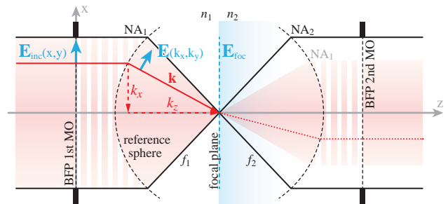
Figure 1. Simplified sketch of the investigated system for parameters n_1 < n_2 and \text{NA}_1 < \text{NA}_2 . An aplanatic high numerical aperture (NA) system is used to tightly focus an incoming beam impinging from left to right. The incoming electromagnetic field \mathbf{E}_{\text{inc}} at the back focal plane (BFP) of the first microscope objective (MO) is projected onto a reference sphere with radius f_1 . A second confocally aligned aplanatic system is used to collect the transmitted light in the second half-space.
