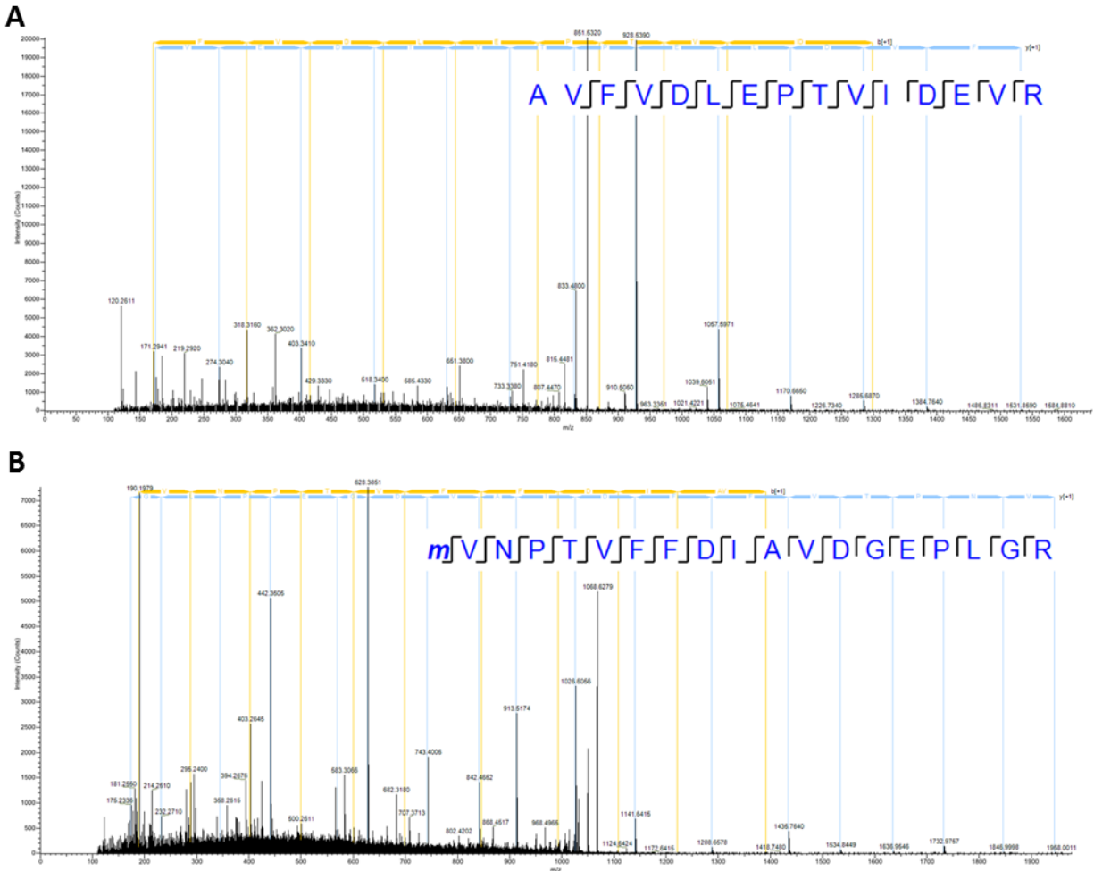
A) LC-MS spectrum of the peptide AVFVDLEPTVIDEVR. B) LC-MS spectrum of the peptide mVNPTVFFDIAVDGEPLGR. Coverage of y- ions (blue) and b- ions (yellow) allowed the identification of the peptides.
