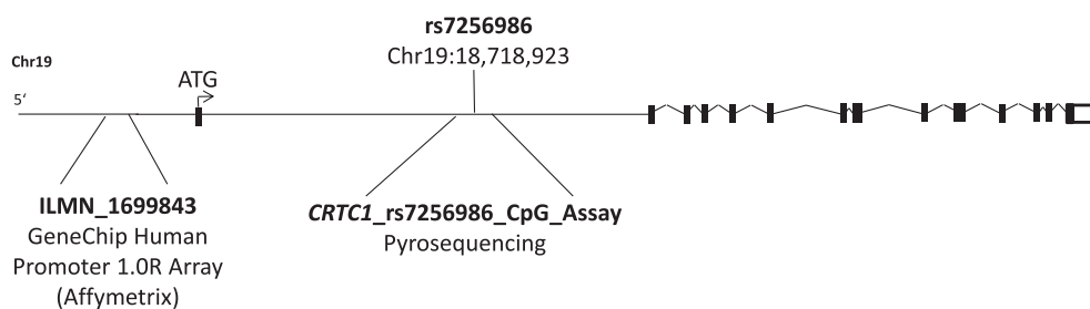
Fig. 1. Schematic representation of the analysed CRTC1 locus. Location of promoter methylation locus (ILMN_1699843 = analyzed illumina probe ID) and CpG Assay for pyrosequencing of rs7256986 (SNP-CpG) and CpG2 is shown. Figure not scaled. Details of the CpG Assay are shown in Table 2. Chr = Chromosome, ATG = translation start site, ILMN = Illumina
