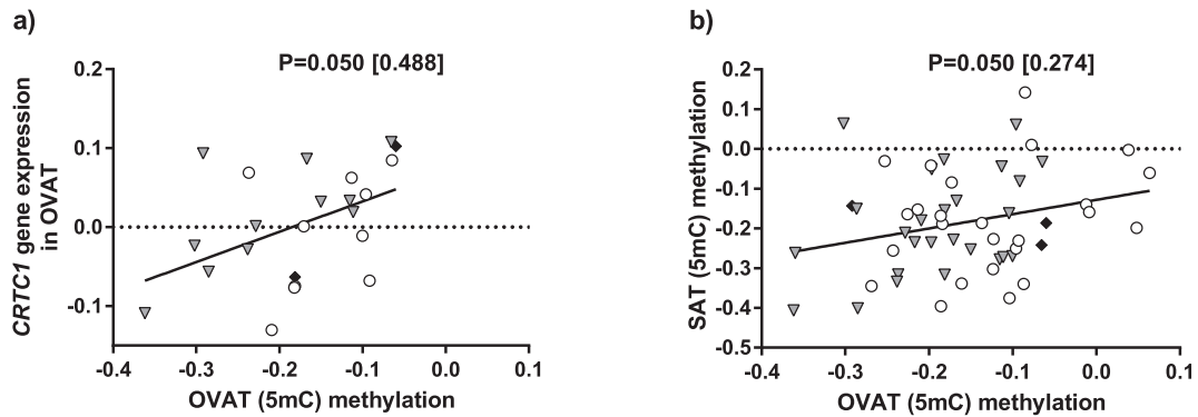
Fig. 5. Correlations of CRTC1 promoter DNA methylation P -values and beta values (in square brackets) were calculated using linear regression models adjusted for age, sex and \ln_{BMI} . OVAT = omental visceral adipose tissue; SAT = subcutaneous adipose tissue; white dots = AA; gray triangles = GA; black diamonds = GG; light gray quarters = no genotype data; N numbers = N a) Correlation of expression with promoter DNA methylation in OVAT ( N = 23) b) Correlation of promoter DNA methylation between SAT and OVAT ( N = 23).
