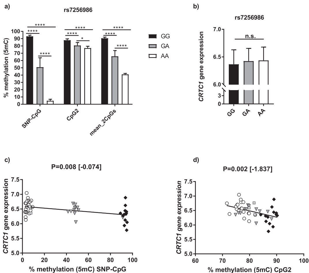
Fig. 2. DNA methylation at SNP-CpG and CpG2 and CRTC1 expression categorized per rs7256986 genotypes in the Sorbs a) DNA methylation at SNP-CpG and CpG2 categorized for genotypes at rs7256986. Data are presented as mean \pm SD. P -values were calculated using independent students t -tests. P -values <0.0001 = **** and <0.005 = *. 5mC = 5-Methylcytosine; Numbers per genotype: GG = 13; GA = 12; AA = 20. b) CRTC1 gene expression stratified per genotypes at rs7256986. Data are presented as mean \pm SD. P -values were calculated using independent students t -tests. Numbers per genotype: GG = 37; GA = 298; AA = 531 c-d) Correlation of CRTC1 expression with DNA methylation at SNP-CpG and CpG2. Data were obtained using linear regression analysis adjusted for age, sex and \ln _BMI; beta coefficient is given in brackets; white dots = AA = 20; grey triangles = GA = 12; black diamonds = GG = 13; light grey quarters = no genotype data.
