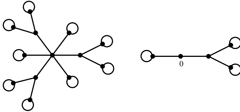
Figure 35: The map on the left represents two polynomials A and B , of degrees 2k = 14 and 3k = 21 respectively, such that \deg(A^3 - B^2) = 9 . Thus, the degree of the difference does not attain its minimum value k + 1 = 8 , but in return both A and B are defined over \mathbb{Q} .
