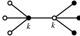
Figure 14: Replace every edge with a three-edge star, and you get the tree I
