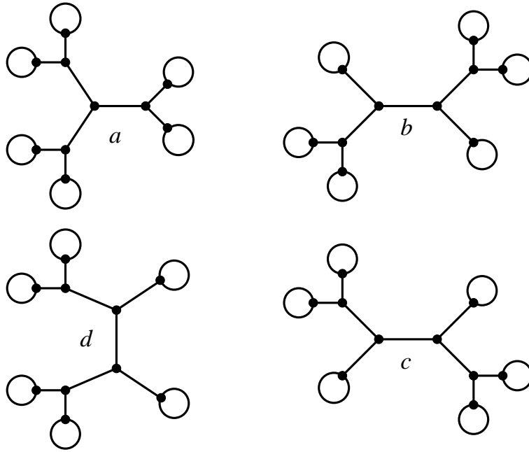
Figure 29: Four trees with the passport (3^{10}, 2^{15}) . The trees a and d are defined over \mathbb{Q} .
