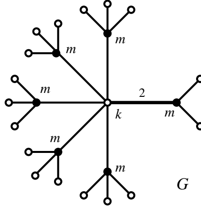
Figure 9: Series G . The degree of the central vertex is k , the number of branches (and the number of black vertices) is k - 1 .
