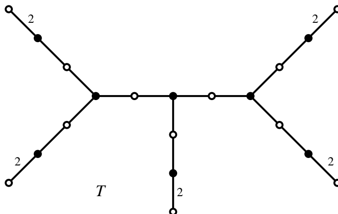
Figure 2: One of the sporadic trees of our classification of unitrees we will speak about further. It is denoted as tree T .
