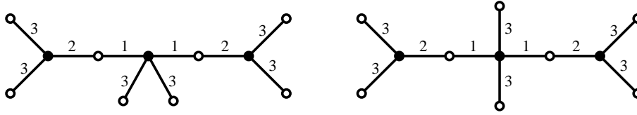
Figure 31: Two trees corresponding to the passport (8^3, 3^8) .
