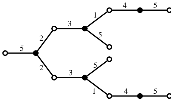
Figure 33: This tree, corresponding to the passport (9^5, 5^9) , is defined over \mathbb{Q} . All known combinatorial invariants of Galois action fail to explain this phenomenon.
