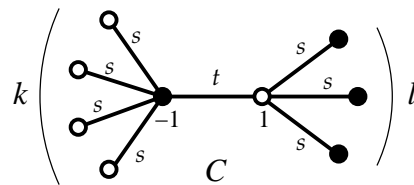
Figure 8: Series C : trees of diameter 3
