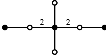
Figure 27: The symmetric tree with the passport (6^1 1^2, 3^2 1^2, 6^1 1^2) .
