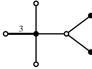
Figure 26: This tree also has monodromy group \mathrm{PGL}_2(7) .
