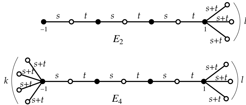
Figure 7: Series E_2 and E_4 : even double brushes
