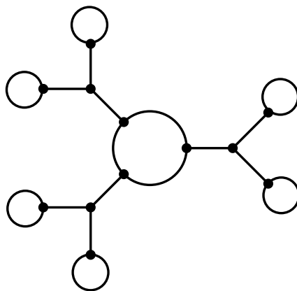
Figure 36: This map represents two polynomials A and B , of degrees 2k = 12 and 3k = 18 respectively, such that \deg(A^3 - B^2) = 9 . Thus, the degree of the difference does not attain its minimum value k + 1 = 7 , but in return both A and B are defined over \mathbb{Q} .
