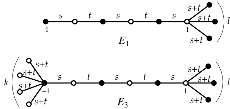
Figure 6: Series E_1 and E_3 : odd double brushes
