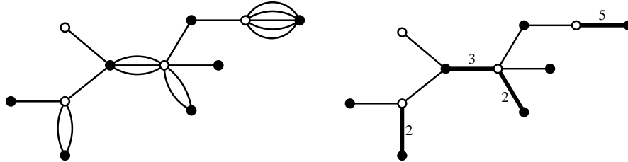
Figure 1: The passage from a map with all its inner faces being of degree 1, to a weighted tree. The weights which are not explicitly indicated are equal to 1; the edges of the weight greater than 1 are drawn thick.
