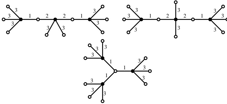
Figure 32: Three trees corresponding to the passport (10^3, 3^{10}) .
