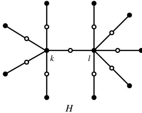
Figure 11: Series H : ordinary trees of diameter 6 which are decomposable.
