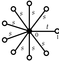
Figure 3: Star-trees. There are k edges of weight s and one edge of weight t , and \gcd(s, t) = 1 .
