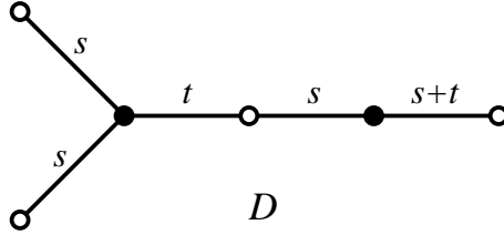
Figure 4: Fork-trees. There are exactly two leaves of weight s and exactly one leaf of weigh s + t . As usual, \gcd(s, t) = 1 .
