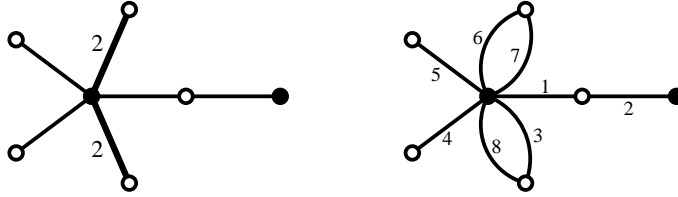
Figure 25: The monodromy group of this tree is \mathrm{PGL}_2(7) . Numbers written on the edges of the tree on the left are their weights; numbers written on the edges of the map on the right are not weights: they are edge labels from 1 to 8.
