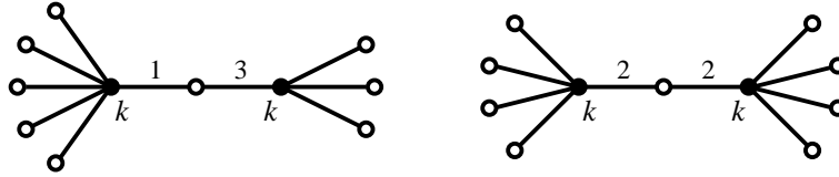
Figure 34: Two trees with the passport (k^2, 4^{12k-4}) . One of them is symmetric, the other one is not.
