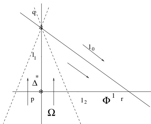
FIGURE 1. Mapping f contracts the line l_1 := \{z_1 = 0\} to the first of its points of indeterminacy q = [0 : 0 : 1] , line at infinity l_0 := \{z_0 = 0\} to the regular point r = [0 : 1 : 0] and do not contracts anything to its second point of indeterminacy p = [1 : 0 : 0] . Levi flat cone = Julia set for f is marked by two punctured lines.
