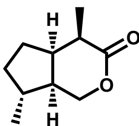
(4 R , 4 aR , 7 R , 7 aS ) - iridomyrmecin or (-) - iridomyrmecin
