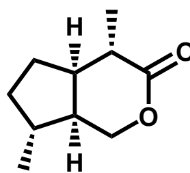
(4 S , 4 aR , 7 R , 7 aS ) - isoiridomyrmecin or (+) - isoiridomyrmecin
