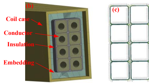
Fig. 3. FE model of 3D shaped control coil (a), mesh of coil section (b) and insulation elements orientation (c).
