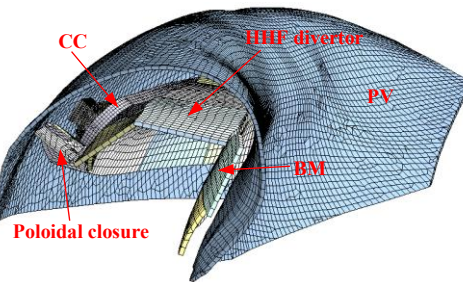
Fig. 2. FE model of simplified divertor volume for CC transient thermal analysis.
