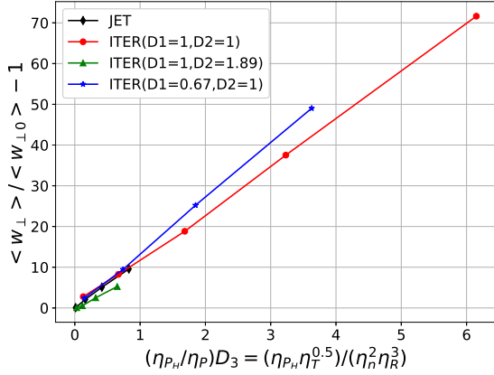
Figure 4. Increase of the volume averaged perpendicular temperature \langle w_{\perp} / w_{\perp}(t = 0) \rangle - 1 in terms of (\eta_{P_H} / \eta_P) D_3 due to the first harmonic ICRF damping using the self-consistent AORSA-CQL3D simulations. For the curves of D_1 = 1 and D_2 = 1 , \eta_{n\phi} = 1.5 and \eta_n = 0.5625 are used. For D_1 = 0.67 , \eta_{n\phi} = 1.0 is used. For D_2 = 1.89 , \eta_n = 2 is used.
