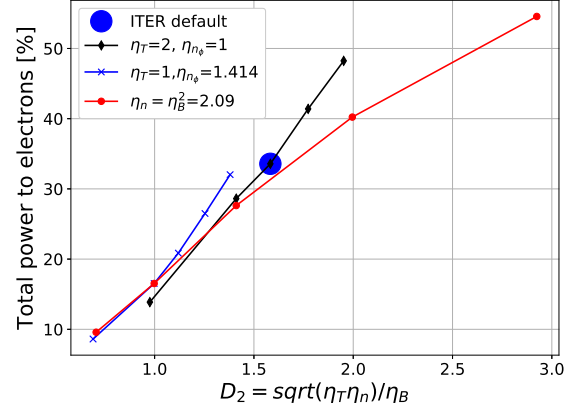
Figure 1. (a) The optimized minority fraction for the maximum ion damping in terms of D_1 . (b) Electron damping percentage in terms of D_2 with the optimized concentration from (a) for ITER. For (a), the density is fixed by the relation of Eq. (1) \eta_n = \eta_B^2 for ITER. For (b), the black and blue lines use the different densities at the same D_1 = 0.49 for ITER, and the red line changes the temperature with the fixed density.
