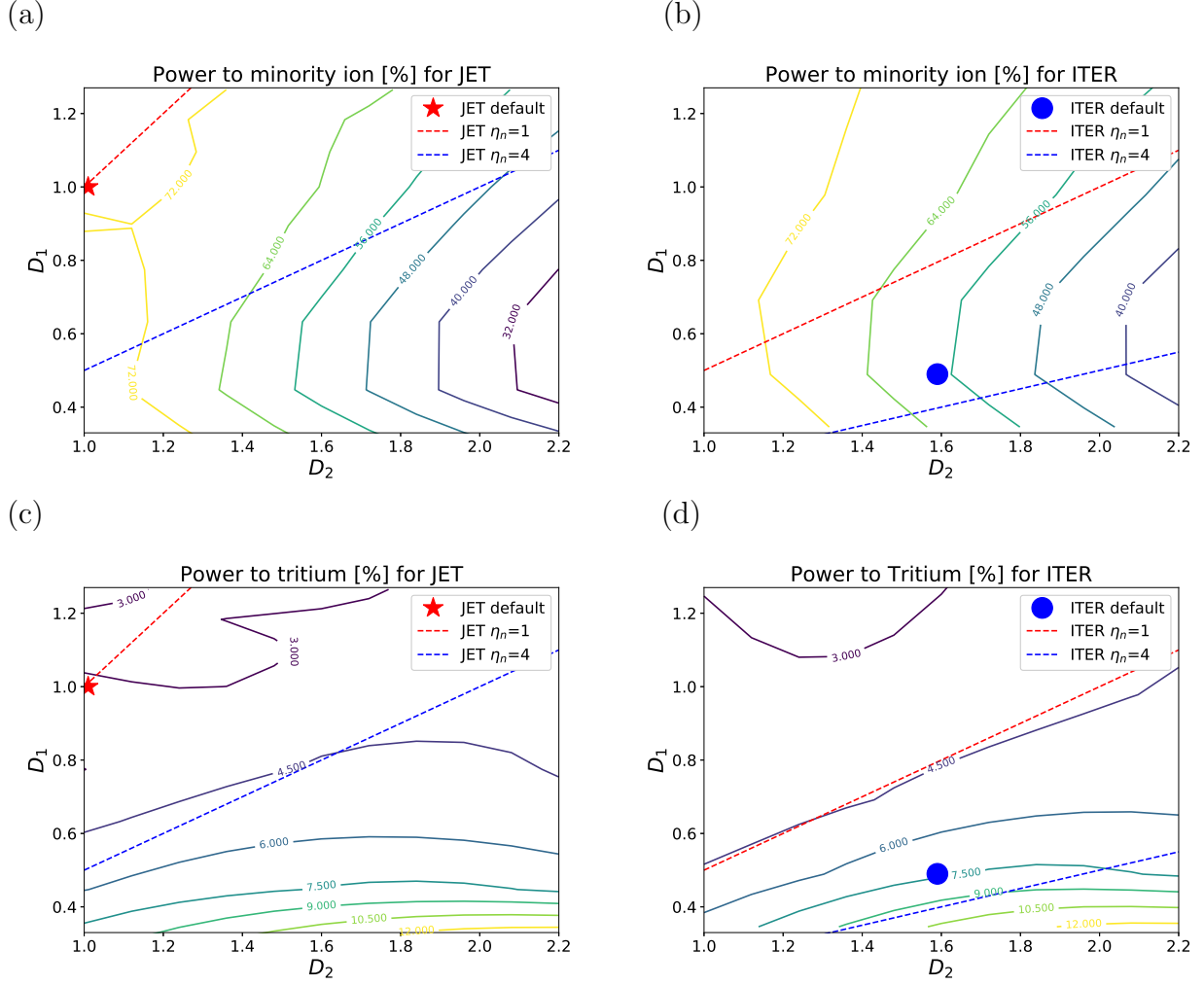
Figure 3. Contour plot of the power partition percentage in terms of D_1 and D_2 at the optimal minority fraction for (a) ^3\text{He} n=1 damping of JET, (b) ^3\text{He} n=1 damping of ITER, (c) Tritium n=2 damping of JET, and (d) Tritium n=2 damping of ITER. D_1 is adjusted by the different temperature \eta_T , and D_2 is adjusted by the different density \eta_n , where \eta_{n,\phi} = 1
