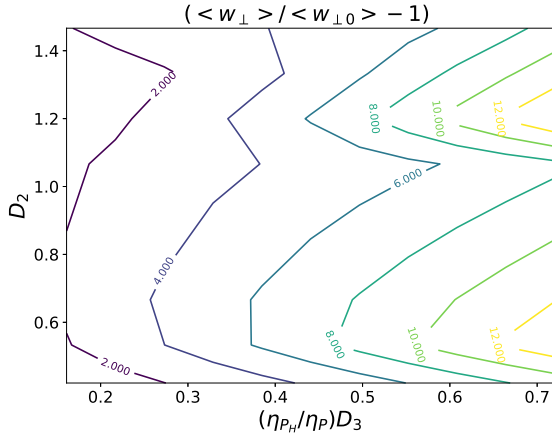
Figure 5. Increase of the volume averaged perpendicular temperature in terms of D_2 and (\eta_{P_H} / \eta_P) D_3 with D_1 = 1 . D_2 is adjusted by the different density \eta_n , and D_3 is adjusted by the different power \eta_P .
