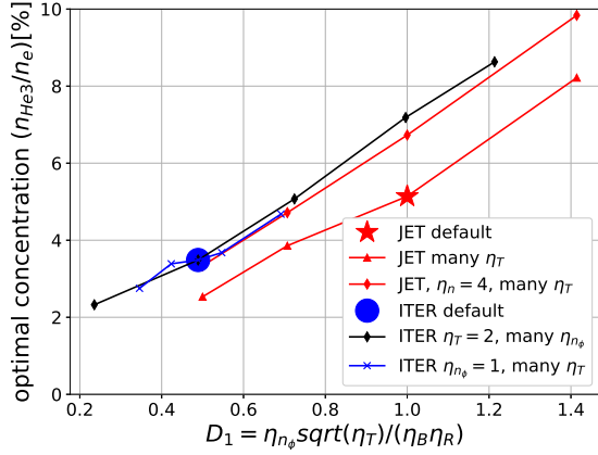
Figure 1. (a) The optimized minority fraction for the maximum ion damping in terms of D_1 . (b) Electron damping percentage in terms of D_2 with the optimized concentration from (a) for ITER. For (a), the density is fixed by the relation of Eq. (1) \eta_n = \eta_B^2 for ITER. For (b), the black and blue lines use the different densities at the same D_1 = 0.49 for ITER, and the red line changes the temperature with the fixed density.
