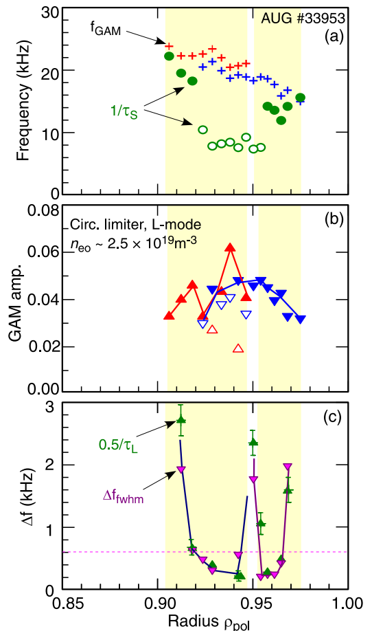
Fig. 5: (a) f_{GAM} & 1/\tau_S , (b) A_{GAM} and (c) GAM width \Delta f_{fwhm} & 0.5/\tau_L profiles for circular, limiter, L-mode #34953.
