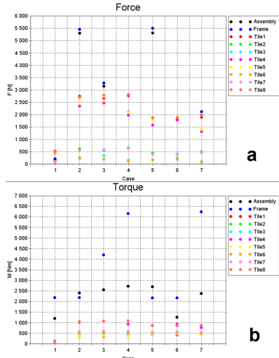
64 Figure 4: Maximal total forces (a) and torques (b) during 65 current quench on assembly, frame and tiles for various 66 cases at \dot{B}_p = 200 T/s 67
