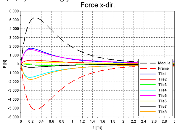
17 Figure 3: Time traces of the force in x-direction acting on 18 the single components for case 5 at at \dot{B}_p = 200 T/s 19
