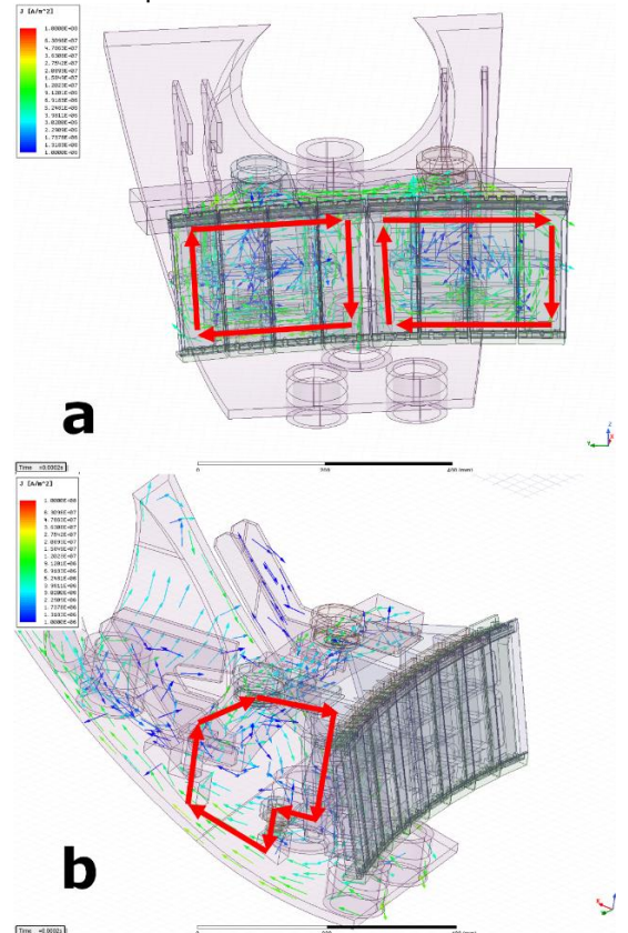
68 Figure 5: Current loops in the cooling plates/tiles (a) and 69 current loops in the assembly/frame (b) for case 3 at \dot{B}_p = 70 200 T/s 71
