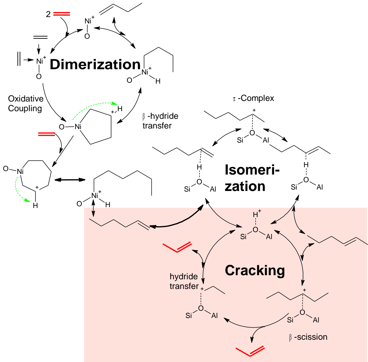
Figure 3: Proposed catalytic mechanism for the propene production from ethene, modifying the mechanism based on the proposal by Iwamoto (Figure 1), considering oligomerization and cracking steps
