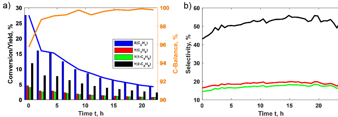
Figure 4: a) Time-dependent values of conversion and yield of the observed products with time on stream and the change in the C-Balance. b) Selectivity of the observable products as a function of time on stream for a reaction of 10% ethene feed at 350^\circ\text{C} , with a W/F=500 \text{ kg}_{\text{Kat}} \cdot \text{s}/\text{m}^3 .
