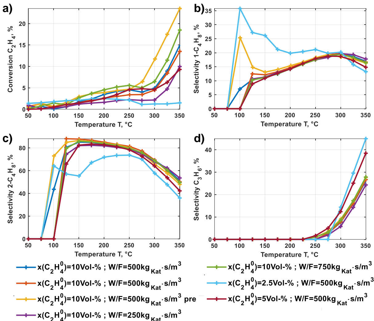
Figure 2: Conversion of ethene (a), selectivity of 1-butene (b), 2-butene (c) and propene (d) over temperature for Ni/(Al)MCM-41 (Si/Al = 60).
