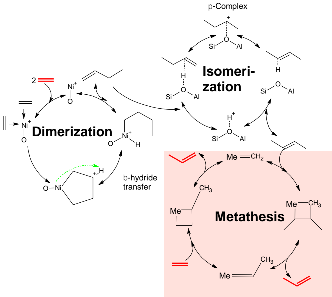
Figure 1: Mechanism of the ethene to propene (ETP) reaction based on the assumed reaction steps by Iwamoto [8].
