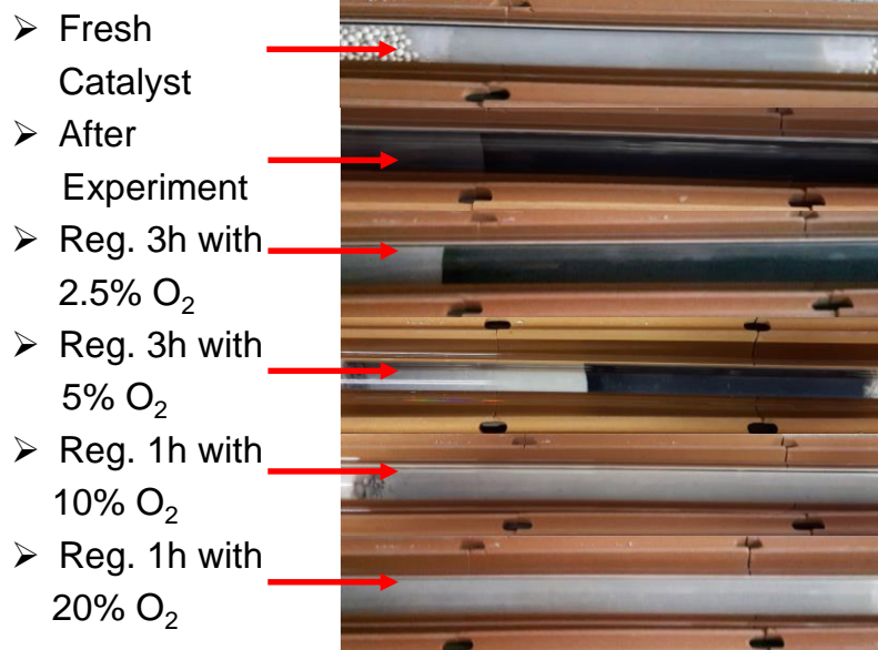
Figure 5: Dependency of the deactivated catalyst bed with varying regeneration time and oxygen concentration.
