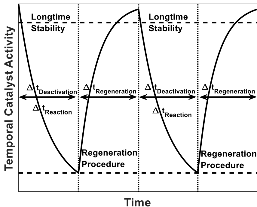
Figure 6: Exemplified cyclic operation of a reactor setup, with distinct reaction and deactivation, subsequently followed by regeneration, with stoppage criteria as low and high activity, initializing the following process step.
