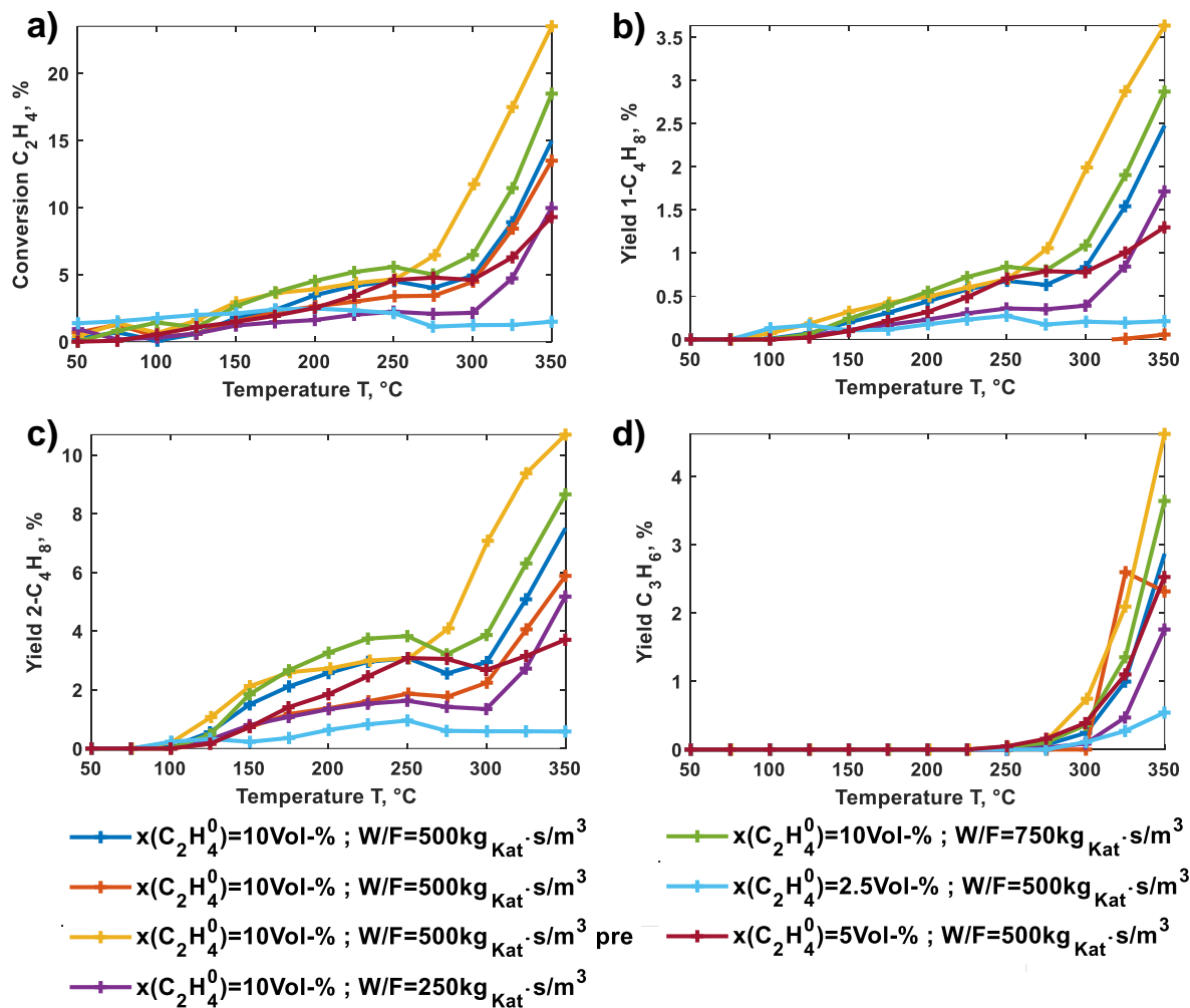
S 1: Conversion of ethene (a), yield of 1-butene (b), 2-butene (c) and propene (d) over temperature for Ni/(Al)MCM-41 (Si/Al = 60).
