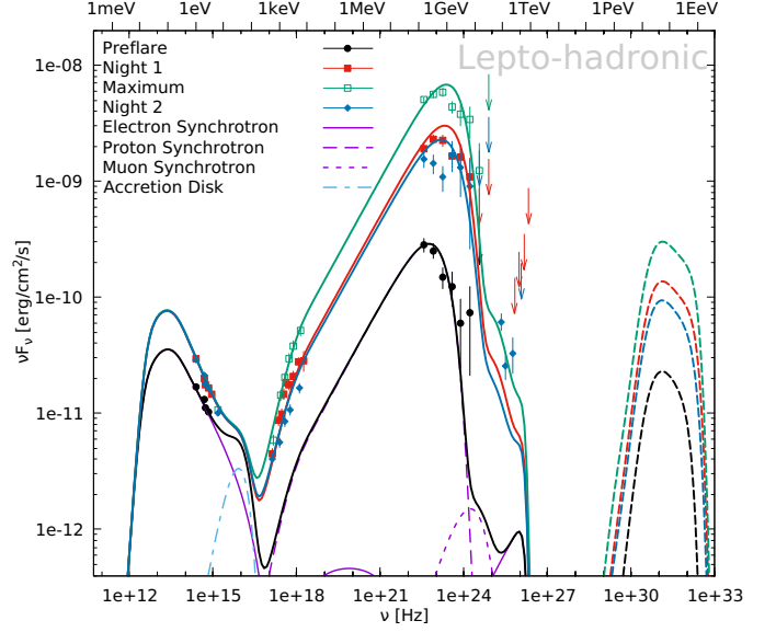
Fig. B.1. Lepto-hadronic model using a larger Doppler factor along with the parameters in Tab. B.1. Data and model lines as in Fig. 8.
