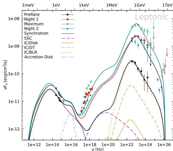
Fig. A.1. Leptonic model using a larger Doppler factor along with the parameters in Tab. A.1. Data and model lines as in Fig. 7.
