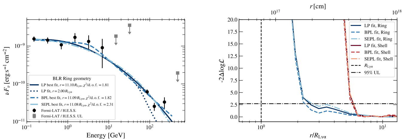
Fig. 6. Left: Best-fit spectra for the BLR ring geometry to the combined Fermi-LAT and H.E.S.S. data. Both data sets are corrected for EBL absorption following Franceschini et al. (2008). The spectral shapes do not change significantly, if the shell geometry is assumed instead. Right: Likelihood profile as a function of the distance r for the different assumed intrinsic spectra and BLR geometries.
