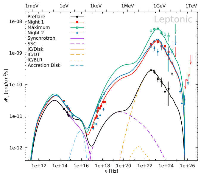
Fig. A.2. Leptonic model using a larger distance from the black hole and a larger Doppler factor. The parameters are given in Tab. A.2. Data and model lines as in Fig. 7.
