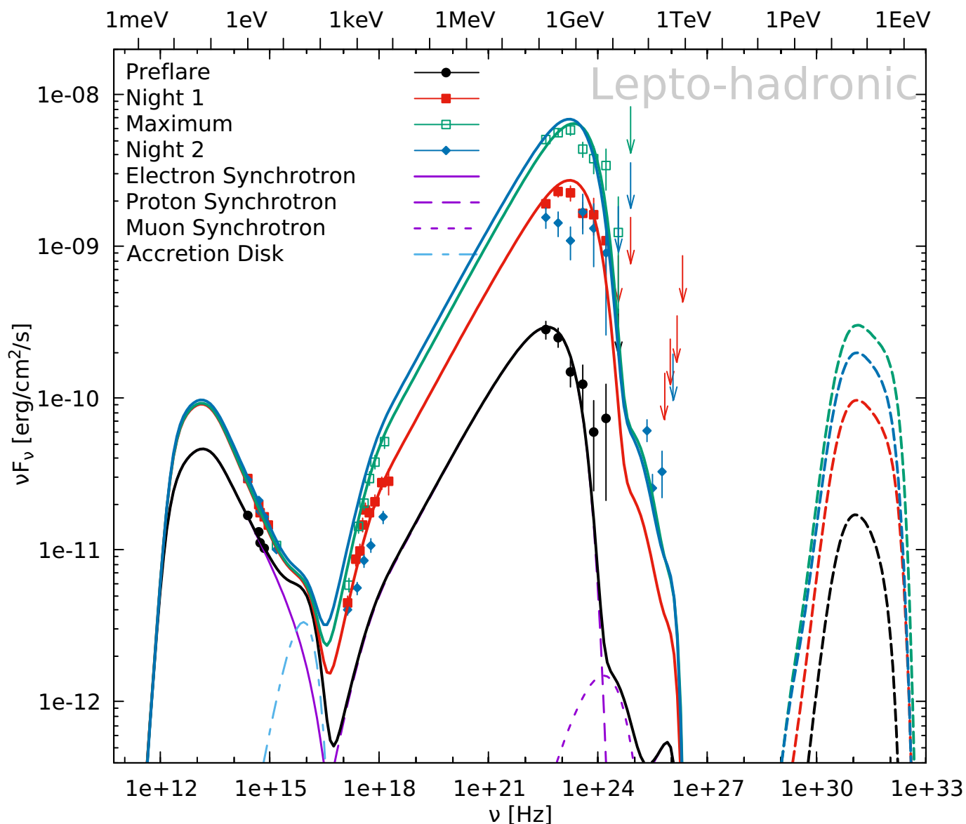
Fig. 8. Multiwavelength spectra and models for the four considered time frames: Preflare (black dots), Night 1 (red filled squares), Maximum (green open squares), and Night 2 (blue diamonds). The \gamma -ray data have been corrected for EBL absorption using the model by Franceschini et al. (2008). The thick solid lines mark the lepto-hadronic photon models, while the thick dashed lines mark the neutrino models. The thin lines mark the spectral components for the Preflare period as labeled.
