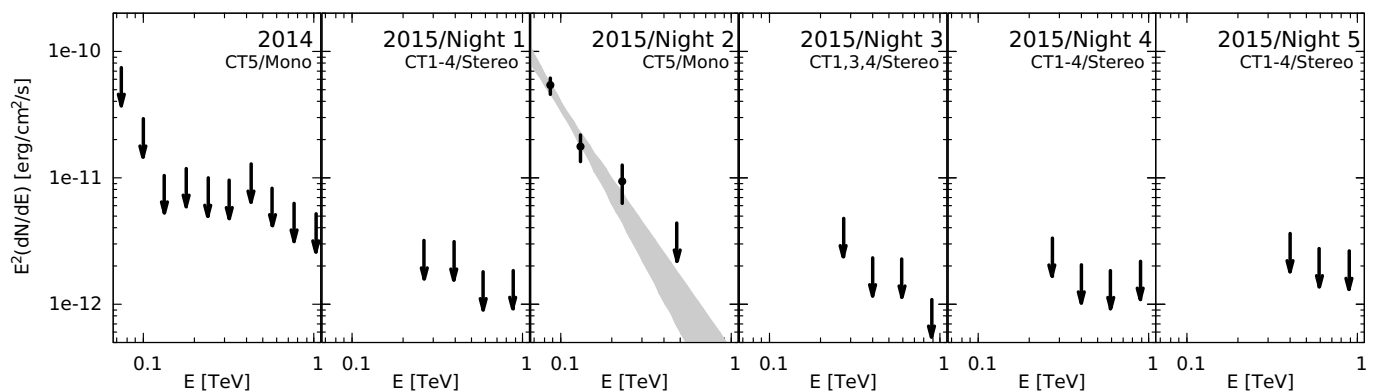
Fig. 1. Observed H.E.S.S. photon spectra for the six data sets as labeled. Arrows mark upper limits (99% confidence level). The gray butterfly is the 1\sigma statistical uncertainty band of the 2015/Night 2 data set. Error bars are statistical only. The second label gives the telescope participation and the analysis used.
