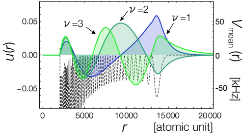
FIG. 6. Radial wavefunctions of the single-particle energy eigenstates for the mean-field Rydberg potential V_{\text{mean}} . Solution \nu = 1 is the most dominant bound state having the largest overlap with the initial single-particle wavefunction. The black dashed curve indicates the spatial profile of the Rydberg potential. The bound-state energies for \nu = 1, 2, 3 modes are -21.5, -13.1 and -3.8 (in the unit of kHz), respectively.
