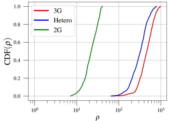
FIG. 8.— Cumulative distribution of network SNR of BNSs in galaxies in Coma cluster measured with various networks of detectors. The binary neutron stars in these galaxies have fixed masses m_1 = 1.45M_\odot and m_2 = 1.35M_\odot and isotropic orbital inclinations.
