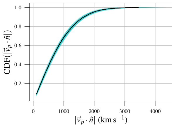
FIG. 7.— Cumulative distribution of magnitude of the line of sight peculiar velocity, |\vec{v}_p \cdot \hat{n}| , of galaxies in the Coma cluster. The cyan curves are 100 realization of sampling radial velocities of galaxies in Coma using halotools and the black curve represents the median.
