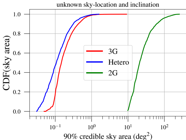
FIG. 11.— Cumulative distribution of 90% credible sky-area of galaxies in Coma cluster measured with various networks of detectors. The binary neutron stars in these galaxies have fixed masses m_1 = 1.45M_\odot and m_2 = 1.35M_\odot and isotropic sky-locations and orbital inclinations. All the sources plotted here have network SNR \geq 10 .
