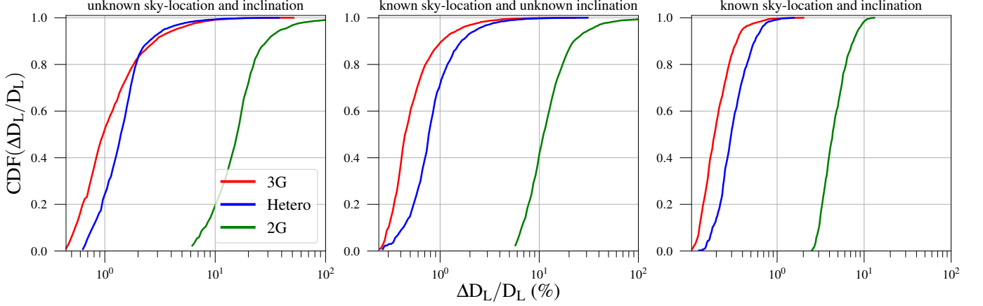
FIG. 9.— Cumulative distribution of 1 - \sigma distance errors of galaxies in Coma cluster measured with various networks of detectors. The binary neutron stars in these galaxies have fixed masses m_1 = 1.45M_\odot and m_2 = 1.35M_\odot and isotropic orbital inclinations. Left panel shows the errors when sky-location and orbital inclination of the binaries are not known to us. Middle panel shows the error when sky-location of the binaries are known and the right panel demonstrates distance errors when both sky-location and orbital inclination of binaries are known. All the sources plotted here have network SNR \geq 10 .
