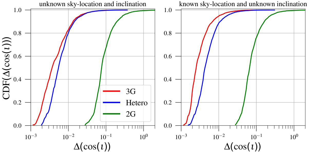
FIG. 10.— Cumulative distribution of 1 - \sigma errors in measurement of orbital inclination of binary neutron stars residing in galaxies in Coma cluster. The binary neutron stars in these galaxies have fixed masses m_1 = 1.45M_\odot and m_2 = 1.35M_\odot and isotropic orbital inclinations. Left panel shows the errors when sky-location and orbital inclination of the binaries are not known to us. Right panel shows the error when sky-location of the binaries are known. All the sources plotted here have network SNR \geq 10 .
