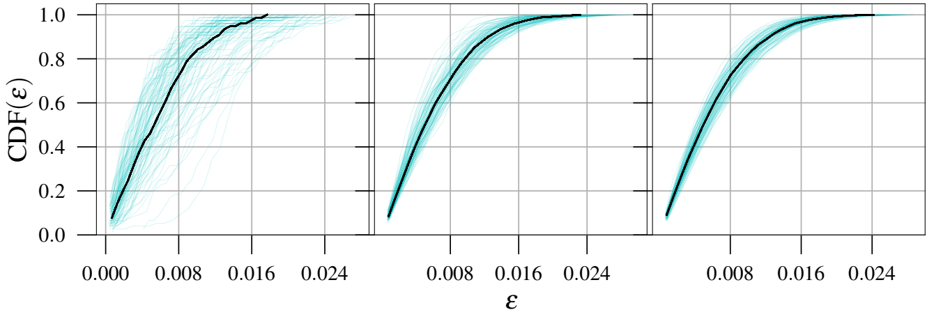
FIG. 6.— Cumulative distribution of \epsilon , the fractional difference between binary neutron star mergers and SNe Ia distances in Coma cluster. The cyan curves are 100 realization of sampling radial positions of galaxies in Coma using halotools and the black curve represents the median. Left, middle and right panels assume that there are 2, 13 and 27 binary neutron star mergers in Coma, respectively.
