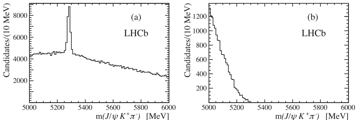
Figure 3: For the P_{B^0 p}^+ \rightarrow J/\psi K^+ \pi^- p decay search (mode I ), the invariant mass of J/\psi K^+ \pi^- combinations in the (a) region above threshold and in the (b) signal region. The peak in the sideband region results from B^0 decays.
