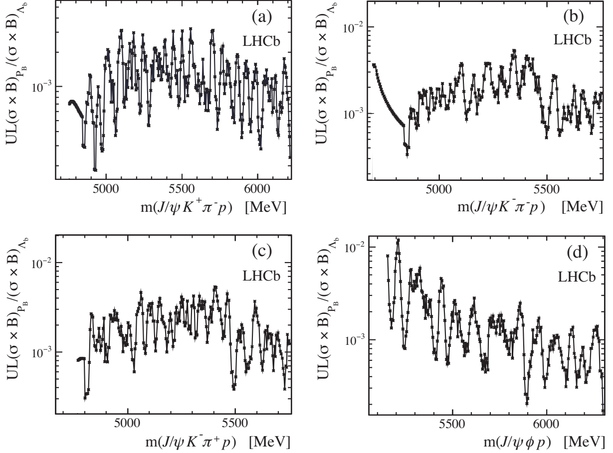
Figure 6: Upper limits on R at 90% CL for (a) J/\psi K^+ \pi^- p , (b) J/\psi K^- \pi^- p , (c) J/\psi K^- \pi^+ p , and (d) J/\psi \phi p final states.
