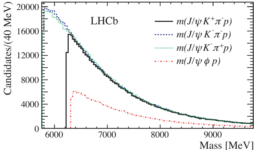
Figure 2: Invariant mass distributions above the decay mass thresholds for the indicated modes.
