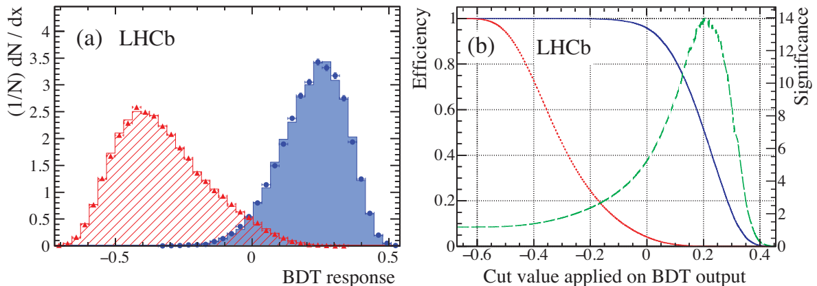
Figure 4: (a) Outputs of the BDT classifier for the J/\psi K^+ \pi^- p final state. The circles (blue) show the signal training sample, and the triangles (red) show the background training sample, while the shaded (blue) histogram shows the signal test sample, and the diagonal (red) line-shaded histogram the background test sample. (b) Efficiencies of signal, solid (blue) curve, and background, dotted (red) curve, and the value of the S/(\sqrt{B} + 1.5) , dashed (green) curve, called “significance,” as a function of the BDT output.
