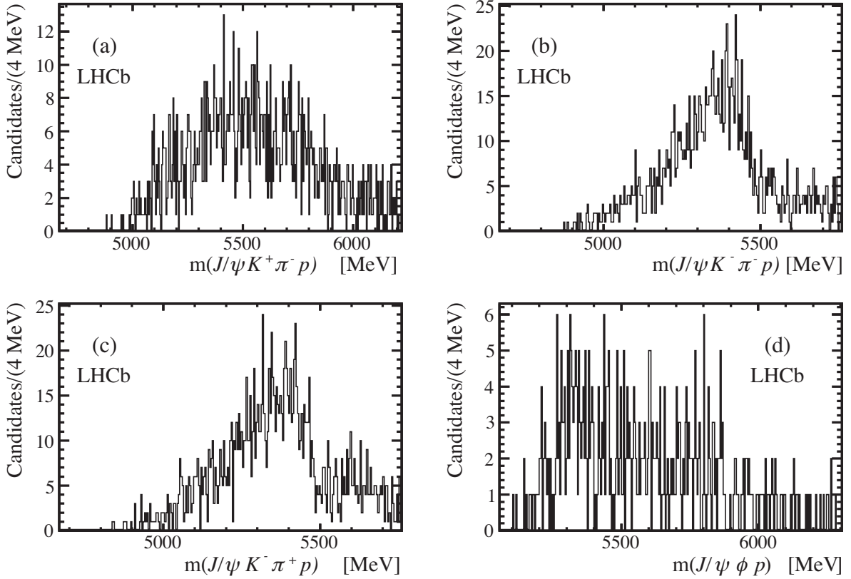
Figure 5: Reconstructed mass distributions after the BDT selection for the (a) J/\psi K^+ \pi^- p , (b) J/\psi K^- \pi^- p , (c) J/\psi K^- \pi^+ p , and (d) J/\psi \phi p final states.
