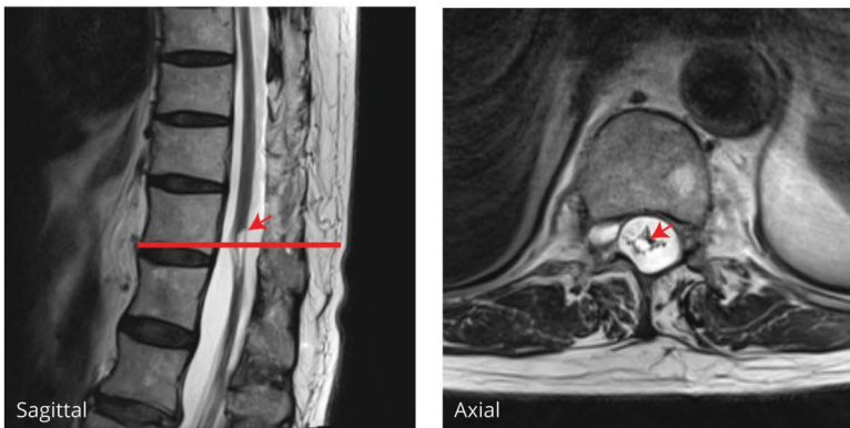
(A) Schematic lesion segmentation including a typical T2W midsagittal slice, which is overlaid with a schematic drawing of the quantitative MRI measures analyzed (lesion area [LA], lesion length [LL], lesion width [LW], ventral midsagittal tissue bridges [VB], and dorsal midsagittal tissue bridges [DB]). (B, C) Representative sagittal and axial images of a patient with traumatic SCI (B) and a patient with ischemic SCI (C) in the chronic phase. The arrows mark the intramedullary cystic cavity.
