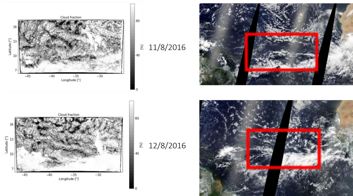
Figure S1. Cloud cover from the model simulations (left column) and MODIS-Terra true color images (right column (Platnick et al., 2003) © NASA) for the 11/8/2016 (upper row) and 12/8/2016 (lower row). The red rectangle represents the model domain.
