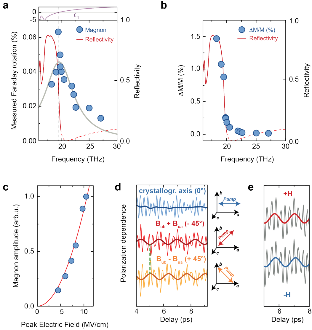
Figure 3 | Pump wavelength, fluence, polarisation and external field dependence at 100 K. (a) Pump wavelength dependence of the measured Faraday rotation and real part of the dielectric function. The blue dots are the values of the coherent magnon amplitude derived from a fit of the oscillations and extrapolated to zero time delay. The solid grey line is a Lorentzian fit intended as a guide to the eye. The solid red curve is the static sample reflectivity measured by Fourier transform infrared spectroscopy (FTIR). The dashed line is a fit to the measured reflectivity. The real part of the dielectric function \epsilon_1 (solid purple line) is retrieved from the reflectivity via a Kramers-Krönig consistent fit. The dotted black line indicates the zero crossing of \epsilon_1 . All the measurements were made at a constant fluence of 20 \text{ mJ/cm}^2 . (b) Pump wavelength dependence of the magnetization change. In order to estimate the absolute change of magnetization we corrected the data of Fig. 1a for the penetration depth mismatch between the pump and the probe (see Supplementary Section 6). (c) Amplitude dependence on the pump field measured at 19.5 THz. The magnon amplitude scales quadratically with the pump electric field - linear with the fluence. Indeed, the electric field ( E ) of a pulse can be estimated from its duration ( \Delta\tau ) and the fluence ( F ) at the sample position. The connecting formula is E = \sqrt{(2F)/(\epsilon_0 c \Delta\tau)} . (d) Pump polarization dependence. Here are presented (light colours) the measured oscillations for different pump polarizations. The darker lines display the same data after application of a numerical low-pass filter (1.5 THz cut-off) to emphasise the magnon (when present). Upper curve: pump polarization directed along one crystallographic axis. Only the Raman-active phonon oscillations ( light blue ) can be detected while the magnon vanishes ( dark blue ). Middle curve: pump polarization in between a and b . The two IR-active phonons are excited with the same initial positive phase ( B_{ub} + B_{ua} ). In addition to the Raman phonons, the magnon appears ( dark red ). Lower curve: pump polarization rotated by 90 degrees, in between -a and b . The two IR-active phonons are excited with phases of opposite signs ( B_{ub} - B_{ua} ). The magnon experiences a \pi phase shift ( dark orange ). (e) External magnetic field dependence. The phase of the magnon does not depend on the initial orientation of the magnetic order.
