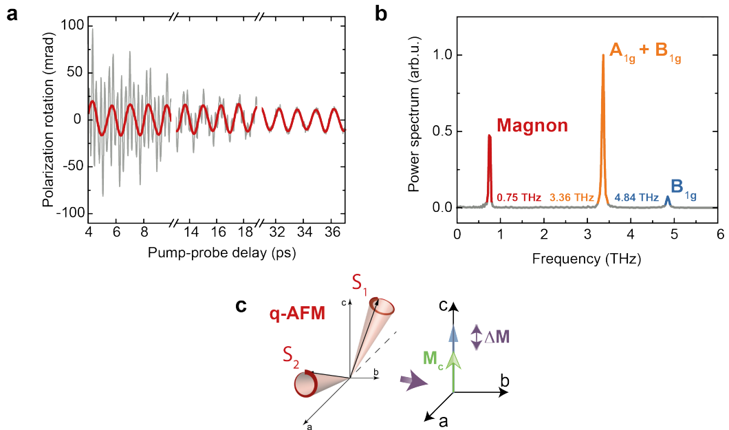
Figure 2 | Transient birefringence measurement. (a) Pump-induced changes in the polarization of the probe as a function of pump-probe delay. The slow-varying component has been subtracted. Multi-component fast oscillations (grey) can be filtered out by a low-pass filter (1.5 THz cut-off) to reveal the slow oscillation associated with the magnon (red). The sample was kept at 100 K while the fluence of the pump pulse was 17.6 mJ/cm 2 . (b) Power spectrum of the oscillatory signal. The three peaks correspond to: 0.75 THz, quasi-antiferromagnetic (q-AFM) magnon (red); 3.36 THz and 4.85 THz, Raman phonons of symmetry A 1g +B 1g (orange) and B 1g (blue), respectively. (c) Cartoon of the spin motion (S 1 and S 2 ) for the q-AFM mode. The small ferromagnetic component along the c axis (green) oscillates in amplitude at the magnon frequency.
