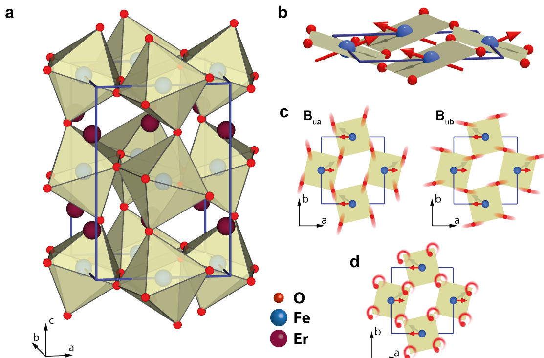
Figure 1 | Structure and magnetic properties. (a) Crystal structure of \text{ErFeO}_3 , an orthorhombically distorted perovskite (Pbnm). (b) Magnetic ordering. The spins of the iron ions order antiferromagnetically along a . Due to the Dzyaloshinskii-Moriya interaction, a canting is induced out of the ab plane resulting in a small ferromagnetic component along c . (c) Eigenvectors of the highest frequency phonons excited by the pump pulse. Singly degenerate infrared active B_{ua} and B_{ub} phonons (calculated eigenvectors for \text{ErFeO}_3 ). (d) The motion of the ions results in an elliptically polarized phononic field due to the non-degenerate nature of the excited IR-active phonons (16.17 THz and 17.03 THz). All Fe-O layers in the unit cell behave in a similar fashion.
