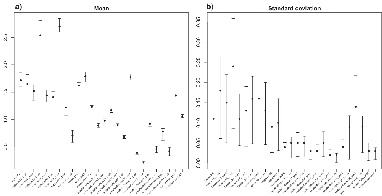
FIGURE 2. NS and MCMC estimates of the mean and standard deviation for some parameters in the Euphorbia data set. The intervals are inferred by using NS and the dots stand for the statistics obtained from the MCMC analysis. All the NS intervals contain the MCMC statistics, suggesting its effectiveness in parameter inference.
