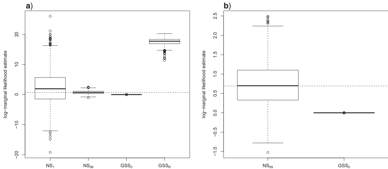
FIGURE A1. NS and GSS marginal likelihood estimates in the statistical example. The subscripts in the NS methods stand for the number of active points, whereas in the GSS method depict the starting value specifications to generate the posterior samples (see text for more details). The horizontal dotted line stands for the true log marginal likelihood value.
