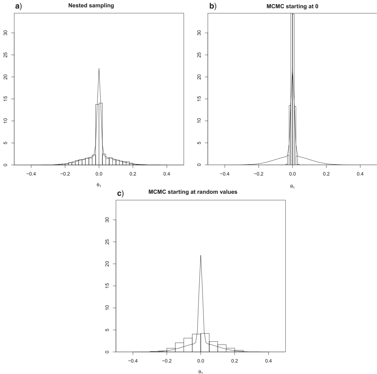
FIGURE A2. The histograms stand for 10,000 posterior samples for the first component of \theta by using nested sampling, and MCMC samples using two different starting values. This behavior is similar in all the components of \theta . The continuous lines depict the true marginal density.
