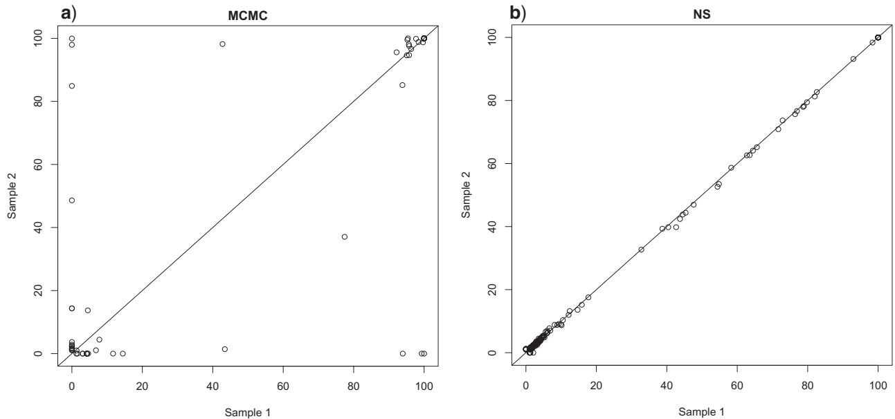
FIGURE 4. Comparison of two MCMC and NS posterior clade probabilities for the Tetrapod data set. The graph on the left shows the difficulty of sampling a parameter space which contain tree islands, where the MCMC chains tend to get stuck and consequently converge to different distributions. The graph on the right shows consistency of NS yielding posterior samples in independent runs, unlike standard MCMC methods.
