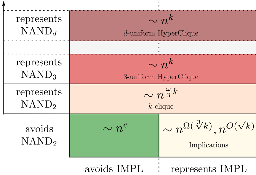
Figure 1: Overview over our main results. The parts of the diagram to the right of the vertical IMPL line depict \mathcal{F} representing IMPL, while the parts to the left avoid IMPL. Analogously, the parts of the diagram above a NAND d line depict NAND d -representing \mathcal{F} , while those below avoid NAND d . For each cell, we illustrate our (typically matching) algorithmic and hardness results, together with a problem that is complete for this cell (in a certain sense). For clarity of presentation, we drop additional f(k)n^c -factors of stated running times.
