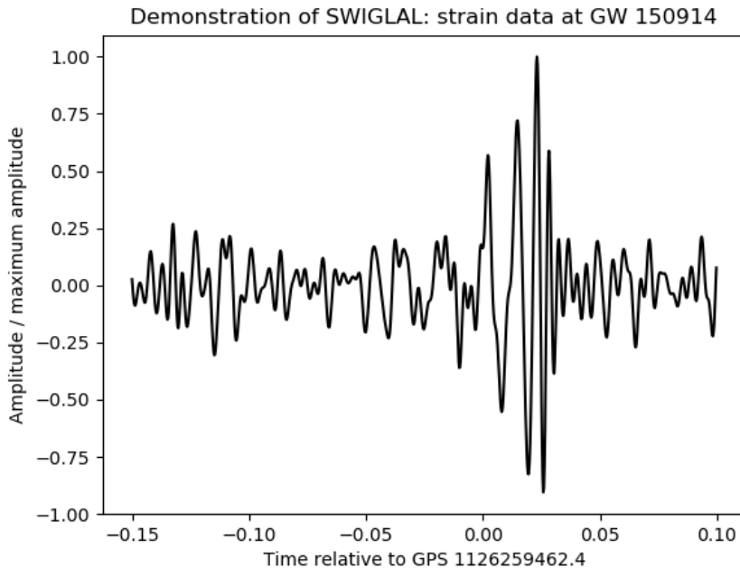
Figure 4: Whitenened, band-pass-filtered strain data from the LIGO Hanford detector at the time of the gravitational-wave event GW 150914 , as output by the example Python script listed in the Appendix.
