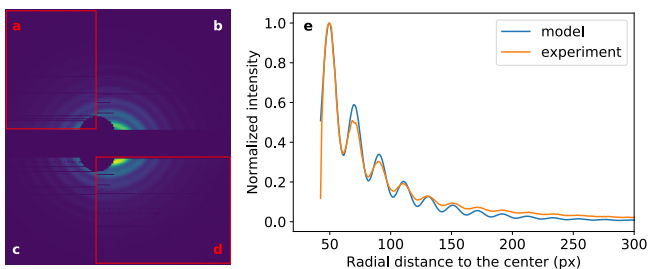
FIG. 2. Sum of 20964 diffraction patterns collected during 220 nm polystyrene injection; experimental data is provided in the red boxes (a, d) and compared to the fitted model. The left figure shows a section of the left half (a) and the right half (d) of the upper detector. The corresponding modeled sections (b, c) are flipped at the horizontal axis to allow for a detailed comparison. (e) Radial plot comparing the angularly integrated experimental and simulated data.
