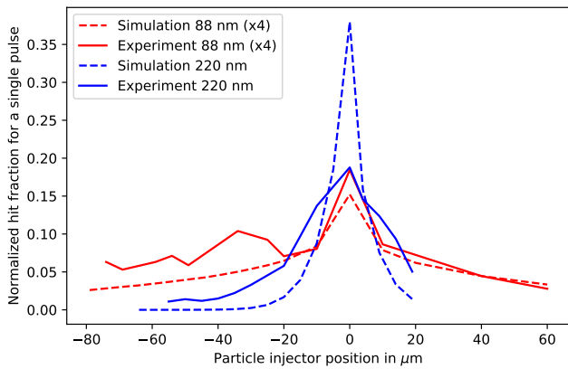
FIG. 4. Measured and simulated hit fraction for a single x-ray pulse dependent on the transverse injector position relative to the x-ray focus. The data for 88 nm polystyrene was scaled by a factor of 4 for better visibility.
