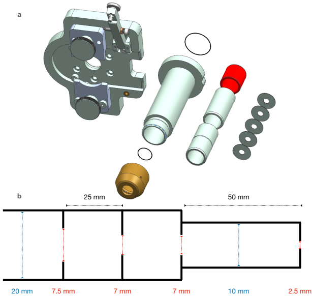
FIG. 1. a) The quick release mount, that attaches the ALS to the aerosol transport tube. The new ALS and its parts. b) The geometry of the ALS set-up used at the experiment at FLASH.
