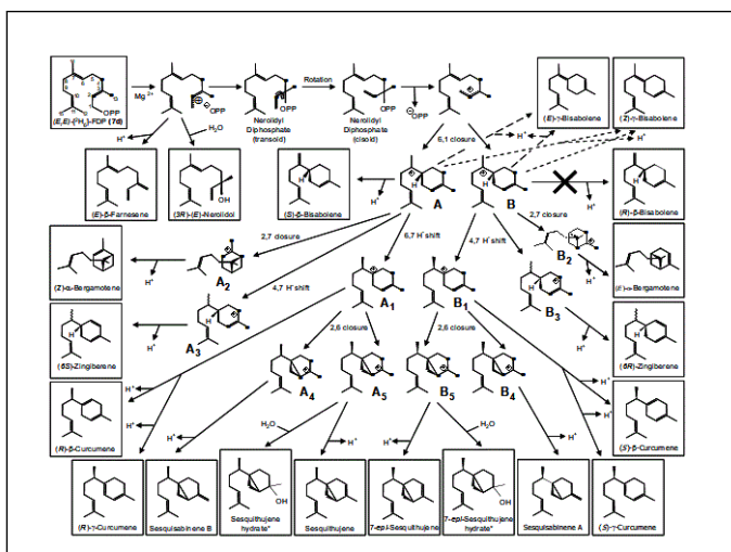
Figure 4C: GC-FID analysis of mono- and sesquiterpenes resulting from incubation of (2E)-GDP and (2E,6E)-FDP with the recombinant terpene synthases TPS4-B73 and TPS5-Delprim. Proposed reaction mechanism for the formation of sesquiterpenes by TPS4 and TPS5 from (2E,6E)-[2H6]-FDP. The scheme is based on previous studies of TPS4 and TPS5.
