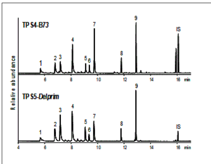
Figure 4B: GC-FID analysis of mono- and sesquiterpenes resulting from incubation of (2E)-GDP and (2E,6E)-FDP with the recombinant terpene synthases TPS4-B73 and TPS5-Delprim. Major sesquiterpenes: (1) 7-epi-Sesquithujene, (2) Sesquithujene, (3) (Z)- \alpha -Bergamotene, (4) (E)- \alpha -Bergamotene, (5) Sesquisabinene A, (6) Sesquisabinene B, (7) (E)- \beta -Farnesene, (8) \gamma -Curcumene*, (9) Zingiberene, (10) (S)- \beta -Bisabolene, (11) \beta -Curcumene*, (12) (E)- \gamma -Bisabolene, (13) 7-epi-Sesquithujene hydrate**, (14) Sesquithujene hydrate**, (15) (3R)-(E)-Nerolidol. IS denotes internal standard. *Stereoisomeric pairs chromatographically not resolved. **Tentatively assigned structure. Unknown cyclic oxygenated sesquiterpenes.
