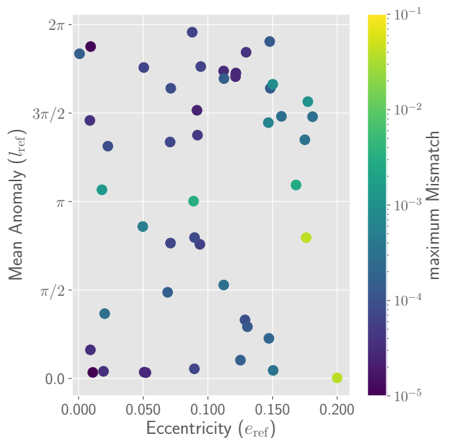
Figure 3. The parameter space covered by the 47 NR waveforms (circle markers) used in the construction of our surrogate model. The axes show the eccentricity and mean anomaly values at t_{\text{ref}} . We also show the dependence of the maximum (over the sky of the source frame) flat-noise mismatches on the parameters eccentricity and mean anomaly (cf. Sec. IV A 2). The colors indicate the maximum mismatch, which systematically increases near the high eccentricity boundary where few training data points are available.
