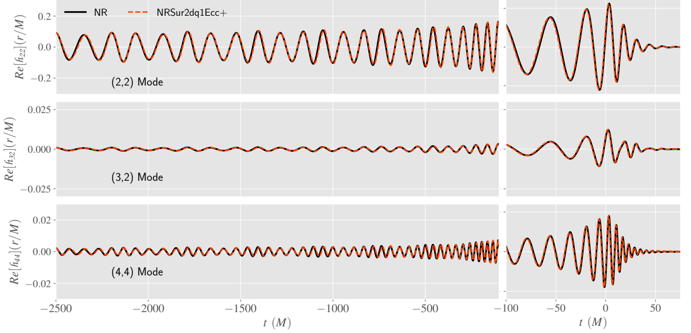
Figure 12. We show the NRSur2dq1Ecc+ prediction (red dashed line) beyond training range ( q = 1 ) of the surrogate for the case that results in the largest mismatch (Fig. 11) in the region defined by e_{\text{ref}} (at t_{\text{ref}} = -2000M ) smaller than \sim 0.05 . We also show the corresponding NR waveform SXS:BBH:1371 (black solid line). The parameters for this waveform are: q = 3 , e_{\text{ref}} = 0.050 and l_{\text{ref}} = 2.45 (at t_{\text{ref}} = -2000M ).
