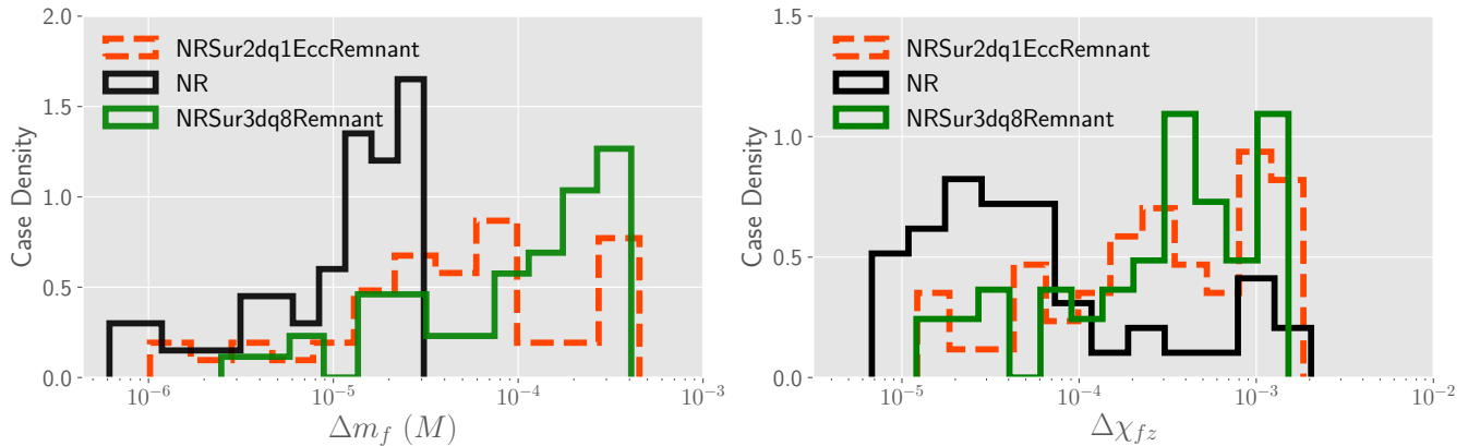
Figure 10. Leave-one-out error histograms of NRSur2dq1EccRemnant (red) for the remnant mass m_f (left) and remnant spin \chi_{fz} (right). For comparison we plot the NR errors (black), estimated by comparing the two highest resolution NR simulations, and errors for the noncentric model NRSur3dq8Remnant (green).
