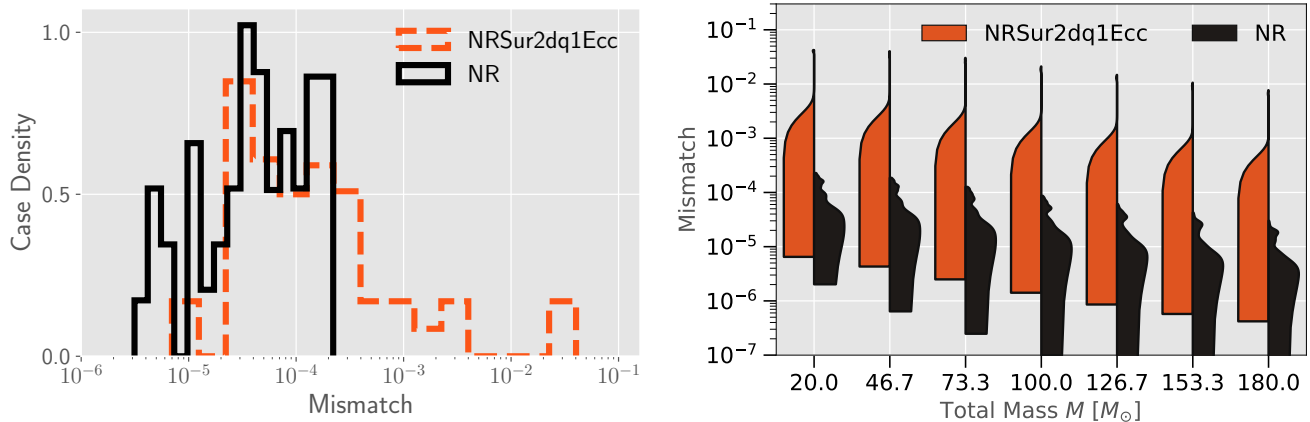
Figure 7. Left panel: Flat noise mismatch between the NRSur2dq1Ecc model (following the leave-one-out validation procedure) and the highest-resolution NR waveform data. For comparison, we also show the NR resolution error, obtained by comparing the two highest available resolutions. Right panel: NRSur2dq1Ecc (validation) mismatches computed using the advanced LIGO design sensitivity noise curve, as a function of the total mass of the binary. For comparison, we also show the NR mismatches. For each mass, the distribution of mismatches are shown as a smoothed vertical histogram (or a violin). The histograms are normalized so that all violins have equal width. The largest errors are found near the parameter domain’s boundary where the trial surrogate, built as part of the cross-validation study, is extrapolating.
