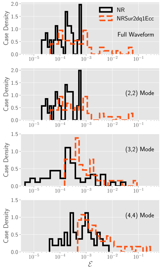
Figure 6. Time-domain leave-one-out errors \mathcal{E} , defined in Eq. (17), for the full waveform as well as the individual modes considered in the model. For comparison, we also show the NR error between the two highest resolutions. The largest errors are found near the parameter domain's boundary where the trial surrogate, built as part of the cross-validation study, is extrapolating.
