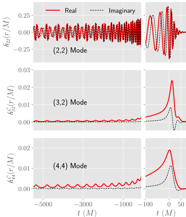
Figure 5. The waveform modes for NR Simulation SXS:BBH:2304 ( e_{\text{ref}} = 0.181 ) are shown. The top panel shows the dominant (2,2) mode in the inertial frame. Two higher-order modes (3,2) and (4,4) in the co-orbital frame are shown in the middle and lower panels respectively. The waveform is aligned such that the peak of the amplitude occurs at t = 0 and the orbital phase is zero at t_{\text{ref}} = -5500M .
