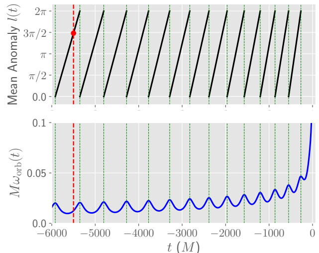
Figure 2. Time evolution of the mean anomaly l(t) (upper panel) and the orbital frequency \omega_{\text{orb}}(t) (lower panel) for the NR Simulation SXS:BBH:2304. Green dashed vertical lines indicate the times for pericenter passages. The anomaly l(t) grows linearly with time over [0, 2\pi) in between two successive pericenters. The red dashed vertical line corresponds to the reference time t_{\text{ref}} = -5500M at which the surrogate model is parameterized.
