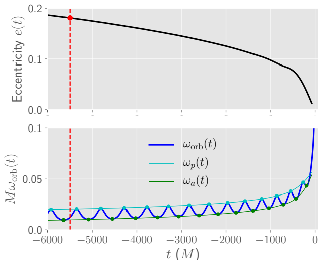
Figure 1. Time evolution of the eccentricity e(t) (upper panel) and the orbital frequency \omega_{\text{orb}}(t) (lower panel) for NR Simulation SXS:BBH:2304. \omega_p and \omega_a denote, respectively, the orbital frequency at pericenter (local maxima, cyan circles) and apocenter passages (local minima, green circles). From this data we construct spline interpolants to obtain \omega_p(t) (cyan curve) and \omega_a(t) (green curve). The eccentricity is then estimated using Eq. (4). The red dashed vertical line corresponds to the reference time t_{\text{ref}} = -5500M at which the surrogate model is parameterized.
