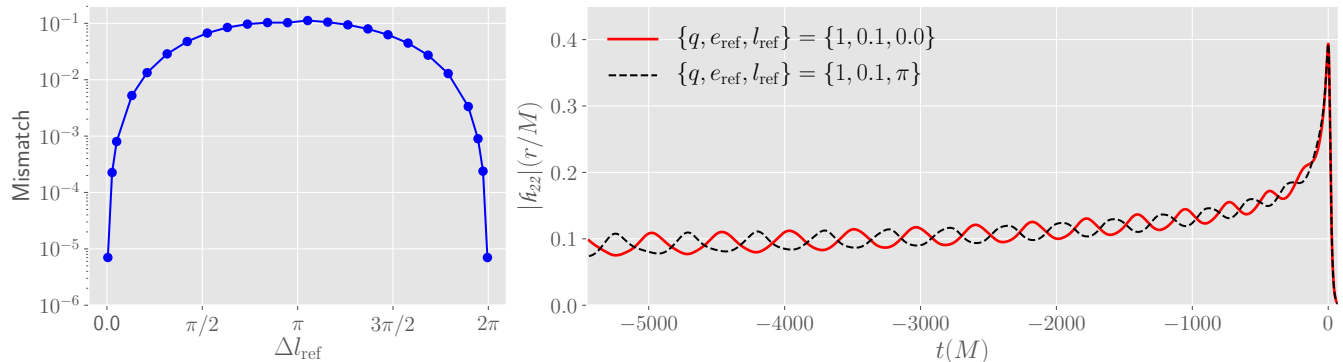
Figure 13. Importance of mean anomaly for waveform modeling and data analysis. Left panel: Flat noise mismatch (optimized over time, phase and polarization angle shifts) between NRSur2dq1Ecc predictions with l_{\text{ref}} = 0.0 and l_{\text{ref}} = \Delta l_{\text{ref}} , at fixed q = 1 and e_{\text{ref}} = 0.1 . While the mismatch, as expected, is \sim 0 for \Delta l_{\text{ref}} = 0.0 and \Delta l_{\text{ref}} = 2\pi , it reaches values \sim 0.1 near \Delta l_{\text{ref}} = \pi . Right panel: The (2, 2) amplitude of the waveforms leading to the maximum mismatch, i.e. l_{\text{ref}} = 0 and l_{\text{ref}} = \pi . These differences cannot be accounted for by a time or phase shift, therefore, mean anomaly is an important parameter to include for waveform modeling and data analysis of eccentric binaries.
