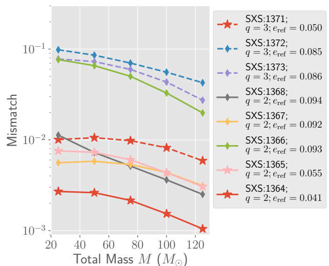
Figure 11. Mismatches against NR for the NRSur2dq1Ecc+ model (a simple extension of NRSur2dq1Ecc ) when the surrogate is evaluated beyond its training parameter range ( q = 1 ). The mismatches are shown as a function of the binary total mass M (at \iota = \pi/3 , \varphi_0 = 0.0 ), and are computed using the advanced LIGO design sensitivity noise curve. We show mismatches for q = 2 ( q = 3 ) as solid lines (dashed lines). We use star markers to denote waveforms with e_{\text{ref}} smaller than \sim 0.05 and diamond markers for the rest. All eccentricity values are computed at a reference time of t_{\text{ref}} = -2000M .
