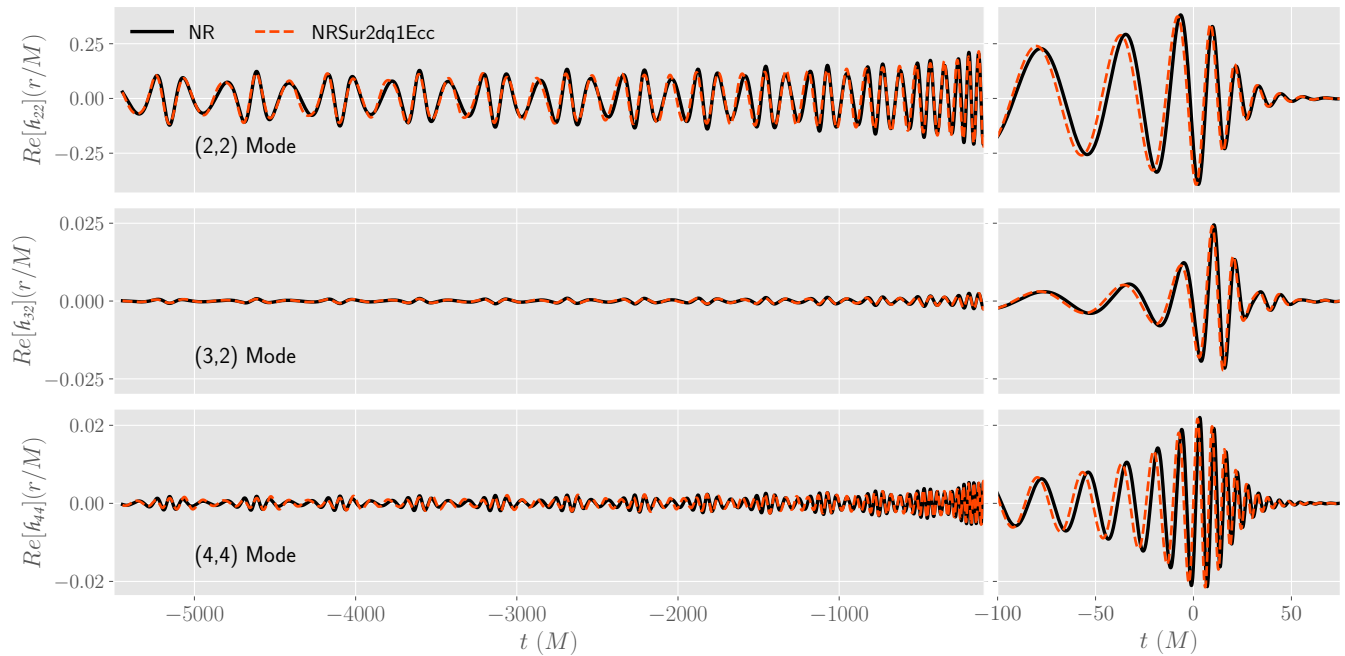
Figure 8. Real part of the waveform modes for the case that results in the largest flat noise mismatch for NRSur2dq1Ecc (red dashed line) in the left panel of Fig 7. We also show the corresponding NR waveform (black solid line). The parameter values for this waveform are: e_{\text{ref}} = 0.176 and l_{\text{ref}} = 2.51 . Note that this plot is generated using a trial surrogate that was not trained using this NR waveform data.
