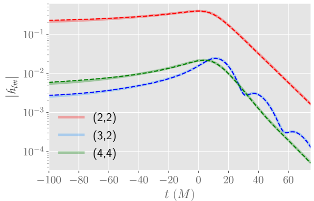
Figure 9. The absolute values of different spherical-harmonic modes are shown as dashed (solid) curves for the surrogate (NR) for SXS:BBH:2308, which has eccentricity e_{\text{ref}} = 0.176 . Mode mixing for the (3, 2) mode is clearly seen in the ringdown signal of the NR waveform and is accurately reproduced by the surrogate.
