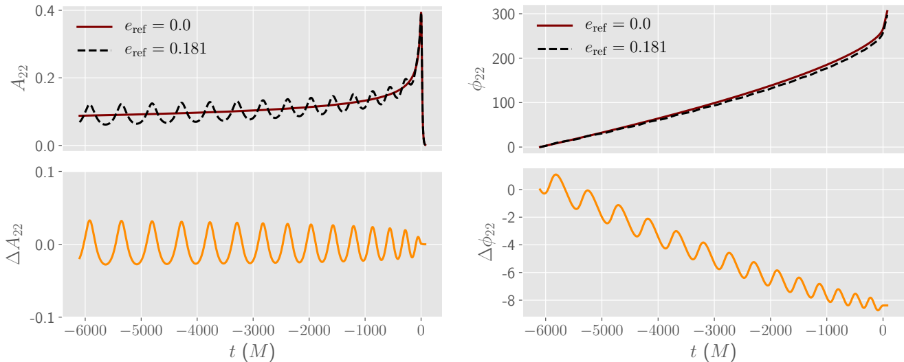
Figure 4. Example decomposition of the amplitude and phase of the (2, 2) mode. Upper left : Amplitude A_{22} of the eccentric waveform SXS:BBH:2304 (with eccentricity e_{\text{ref}} = 0.181 ) along with the amplitude A_{22}^0 of the noneccentric waveform SXS:BBH:1155. Lower left : The residual amplitude \Delta A_{22} = A_{22} - A_{22}^0 . Upper right : Phase \phi_{22} of the eccentric waveform SXS:BBH:2304 and the phase \phi_{22}^0 of the noneccentric waveform SXS:BBH:1155. Lower right : The residual phase \Delta\phi_{22} = \phi_{22} - \phi_{22}^0 . In this work we model \Delta A_{22} and \Delta\phi_{22}
