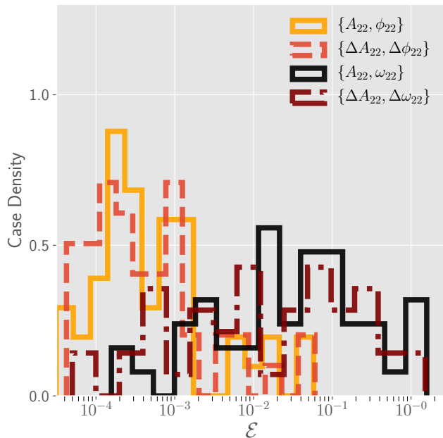
Figure 14. Histograms of surrogate errors (defined in Eqs. (17)) for the four different decomposition strategies we consider. We find that modeling the residual amplitude \Delta A_{22} and residual phase \Delta \phi_{22} yields the least errors.
